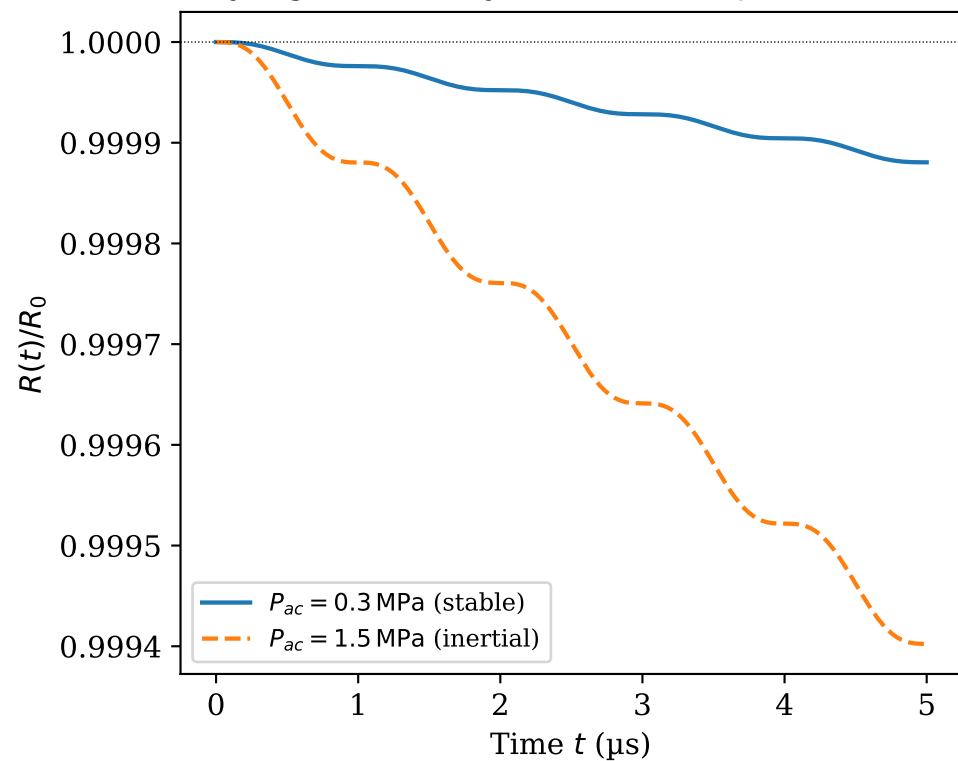
Rayleigh-Plesset dynamics, R_0 = 2\text{ }\mu\text{m} , f = 1\text{ MHz}
