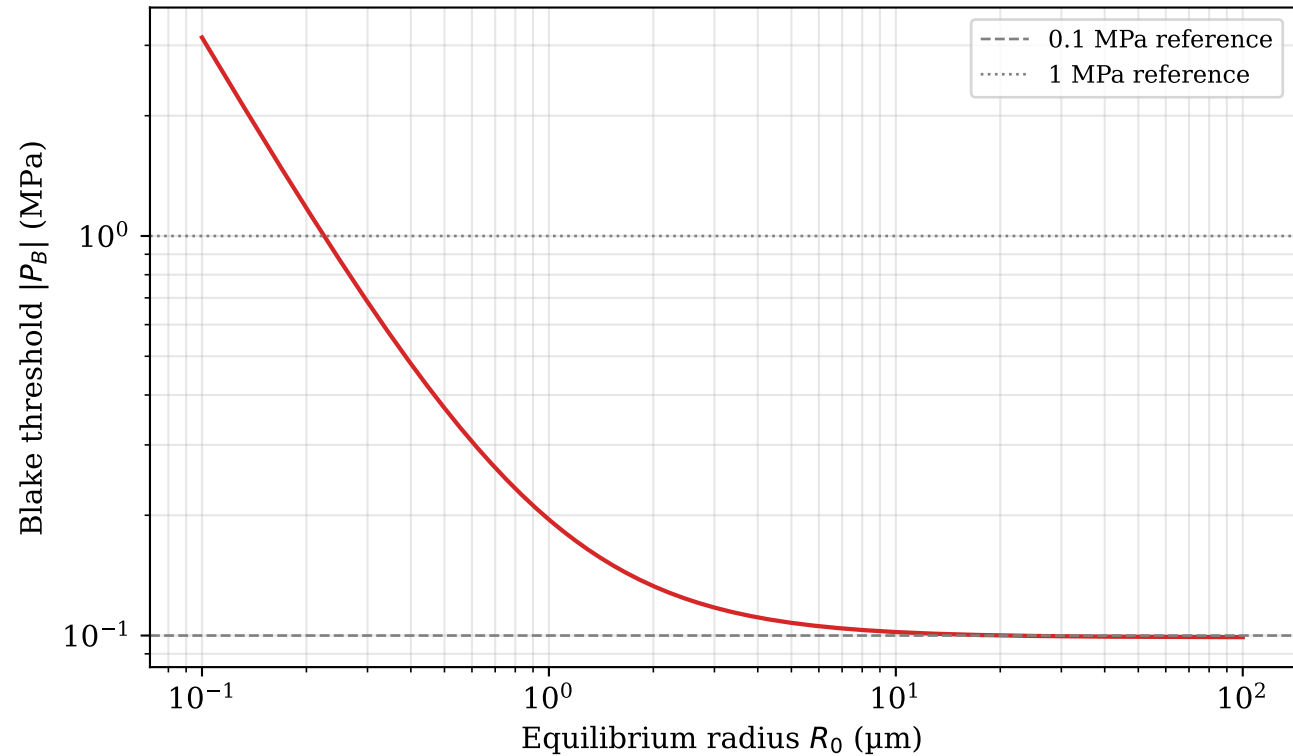
Blake inertial cavitation threshold vs bubble radius
