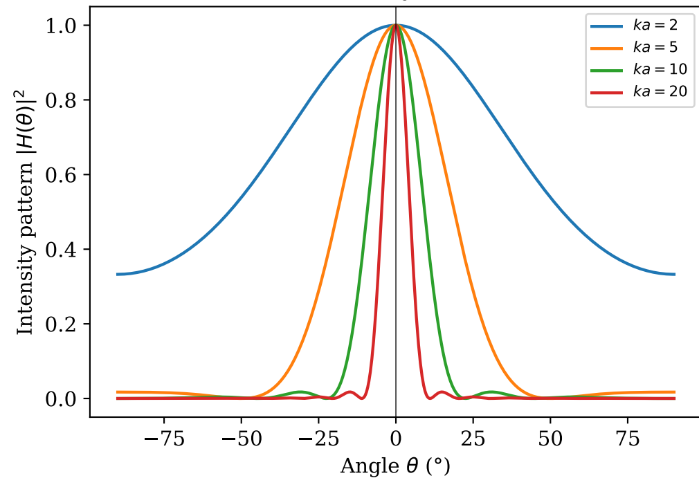
Piston directivity (linear scale)
