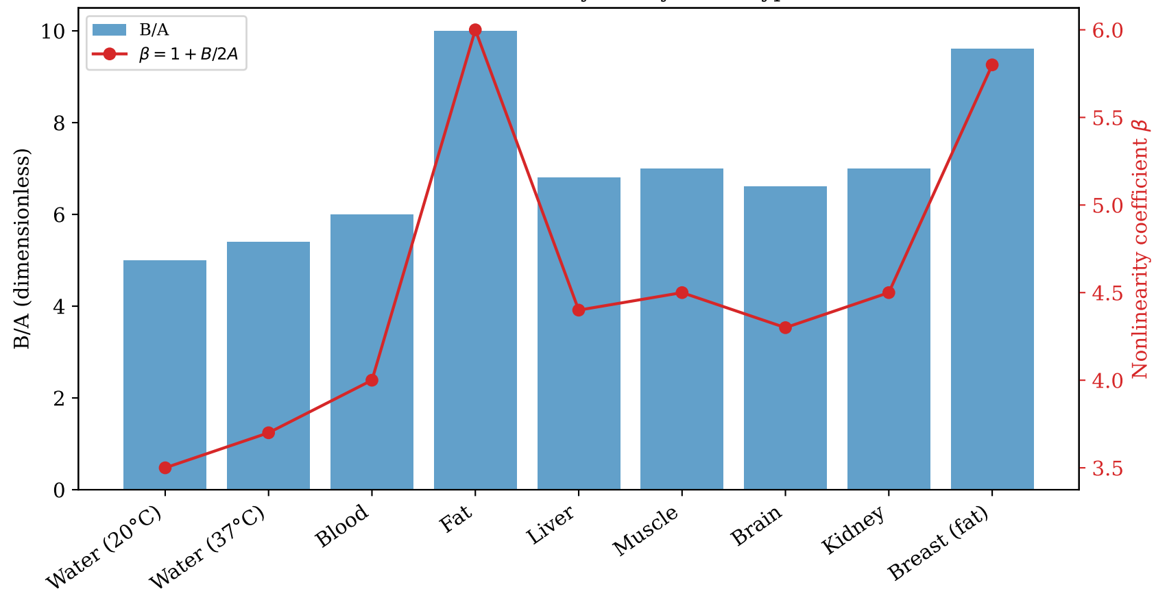
Acoustic nonlinearity B/A by tissue type
