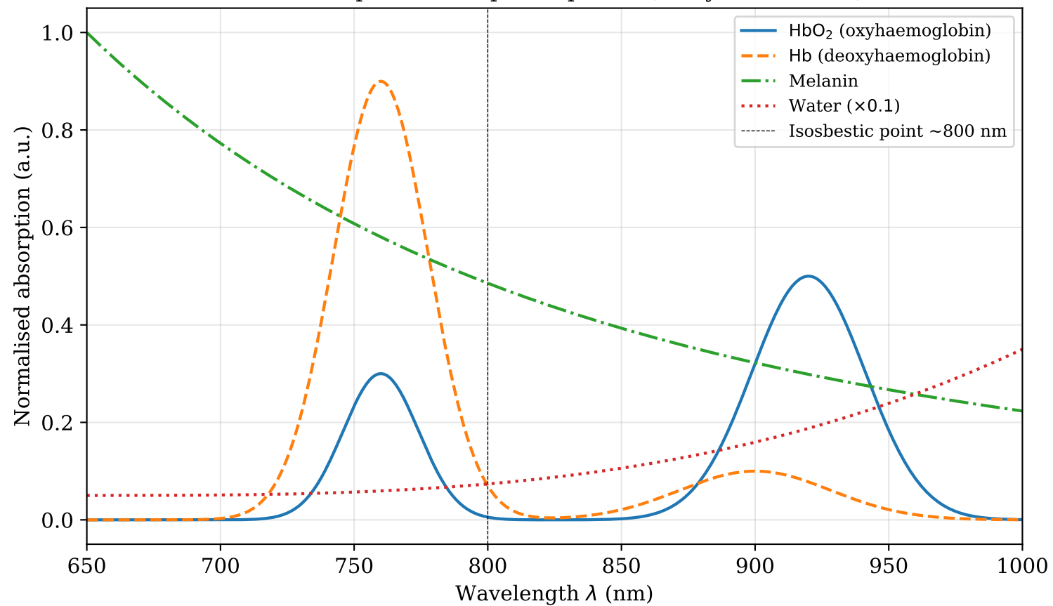
Near-IR optical absorption spectra (analytical models)
