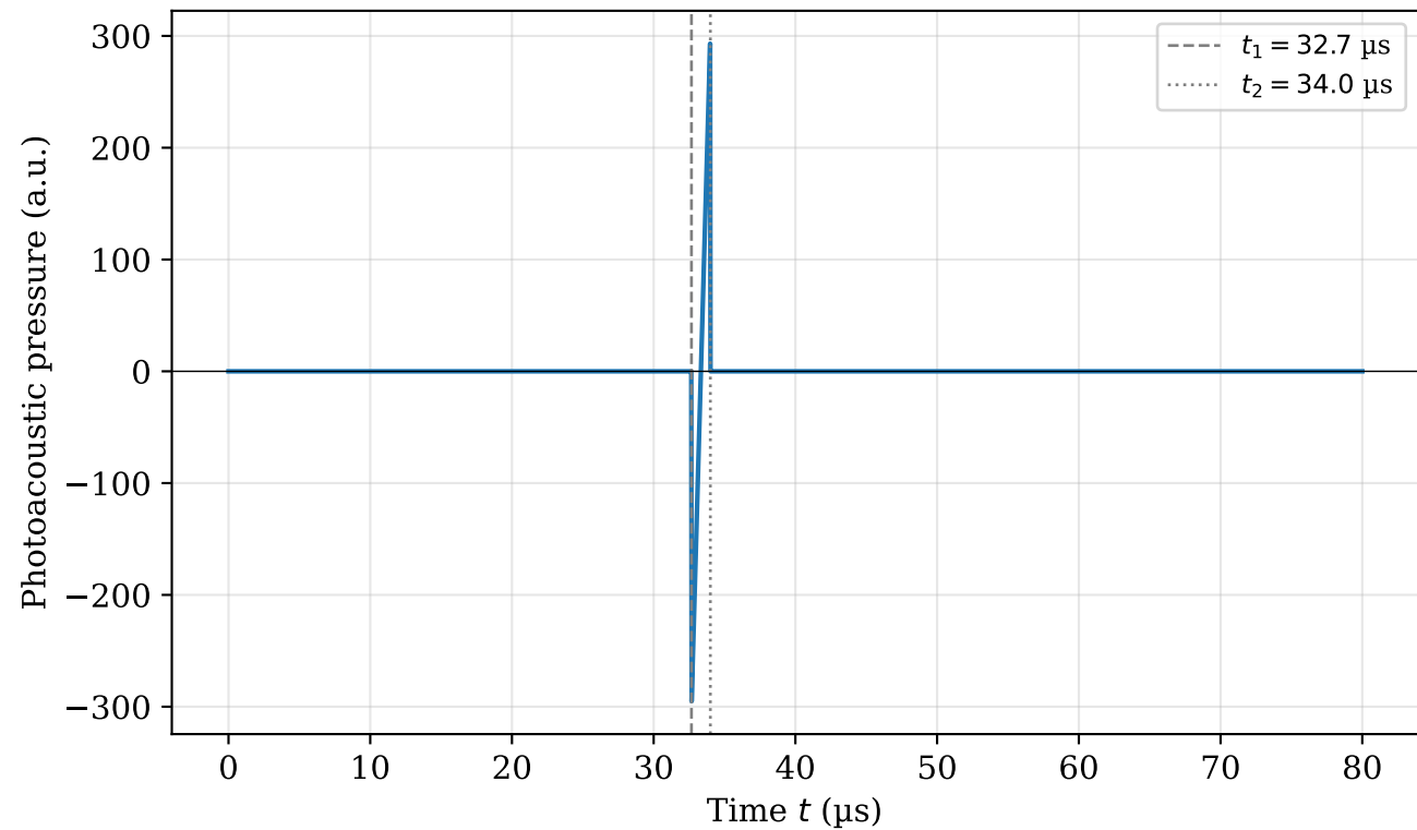
PA signal from spherical absorber ( R = 1.0 mm, r_d = 50 mm)
