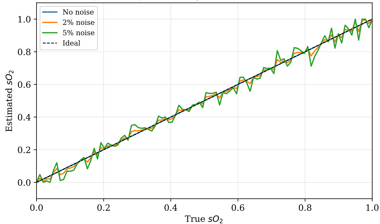
Spectroscopic unmixing: HbO 2 /Hb at 760/850 nm
