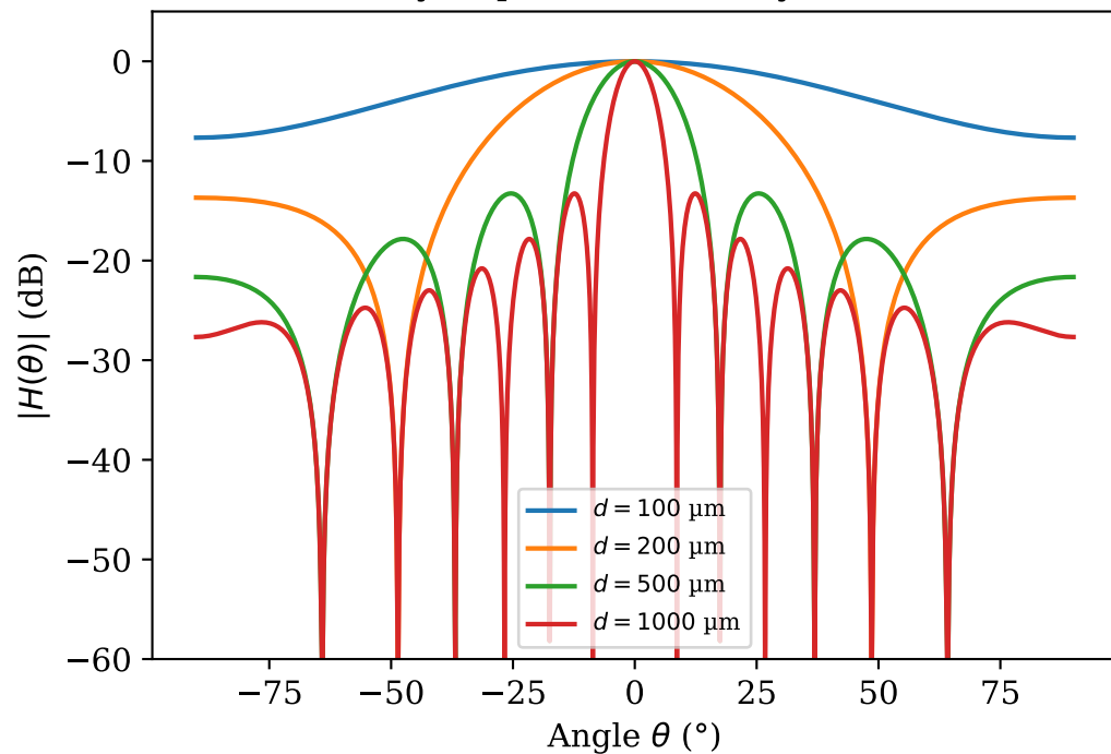
Hydrophone directivity (dB)
