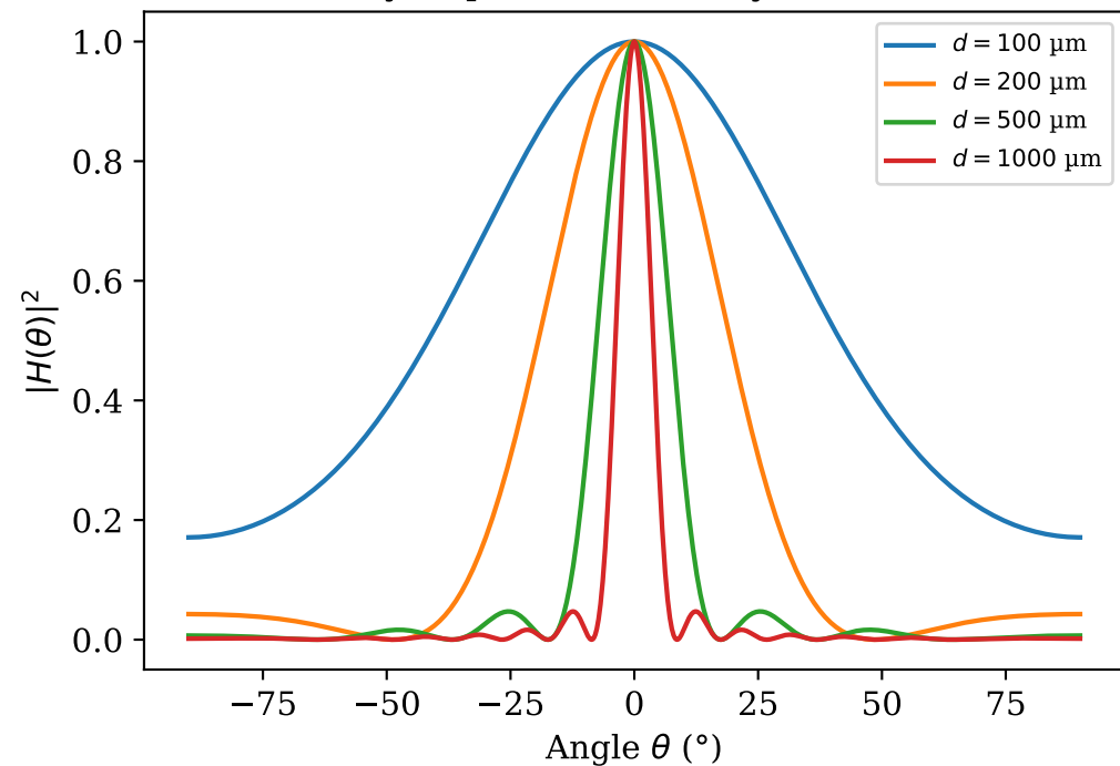
Hydrophone directivity (linear)
