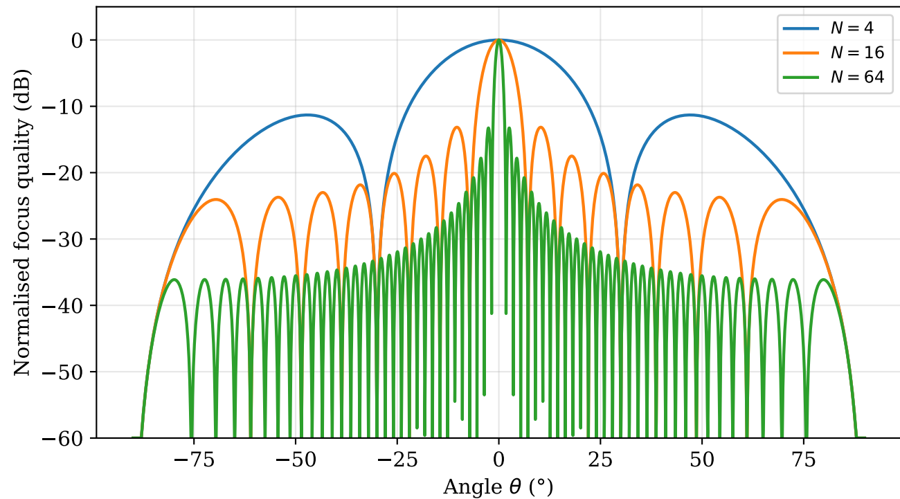
Time-reversal focus quality vs array size d = \lambda/2 , coherent gain = 20\log_{10} N dB
