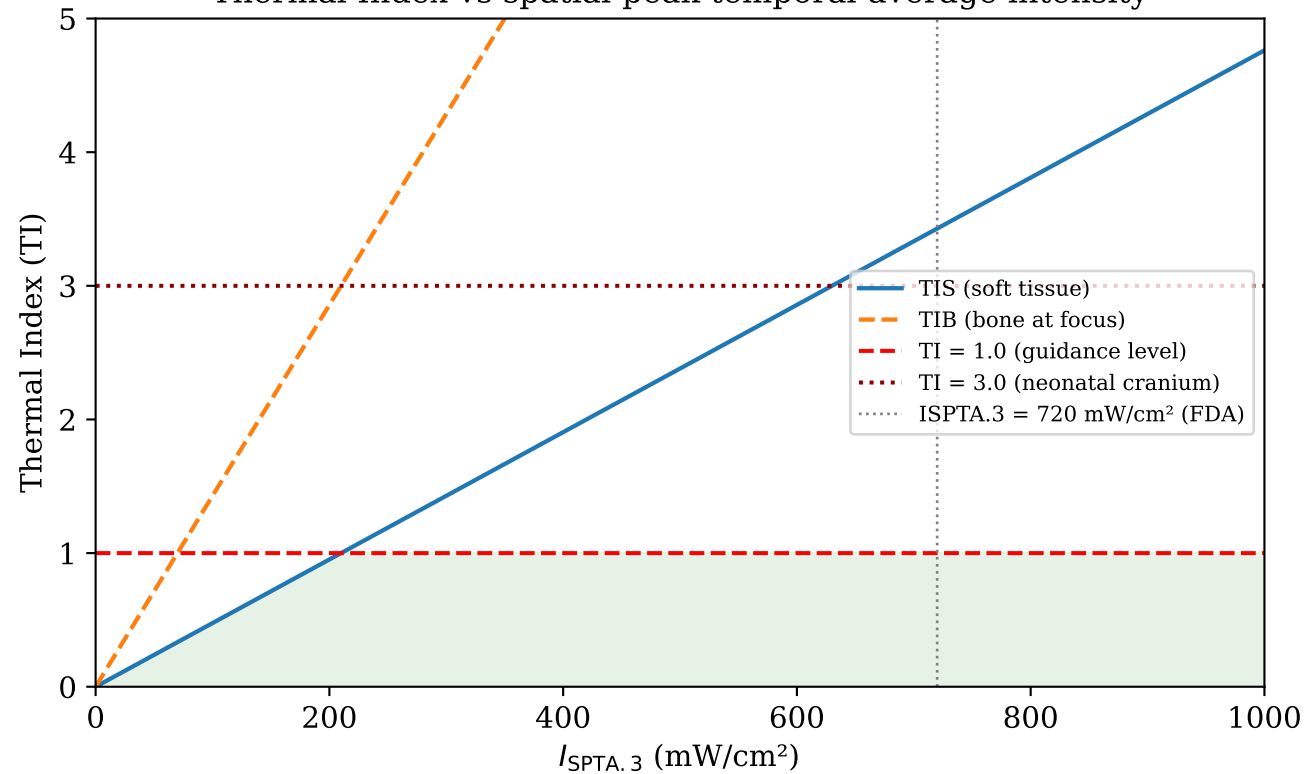
Thermal Index vs spatial-peak temporal-average intensity
