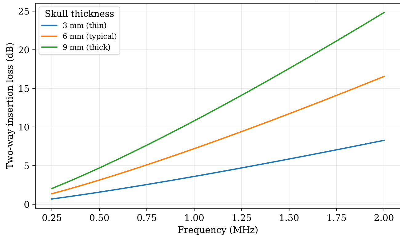
Skull insertion loss: \alpha(f) = \alpha_0 f^{1.2} , two-way
