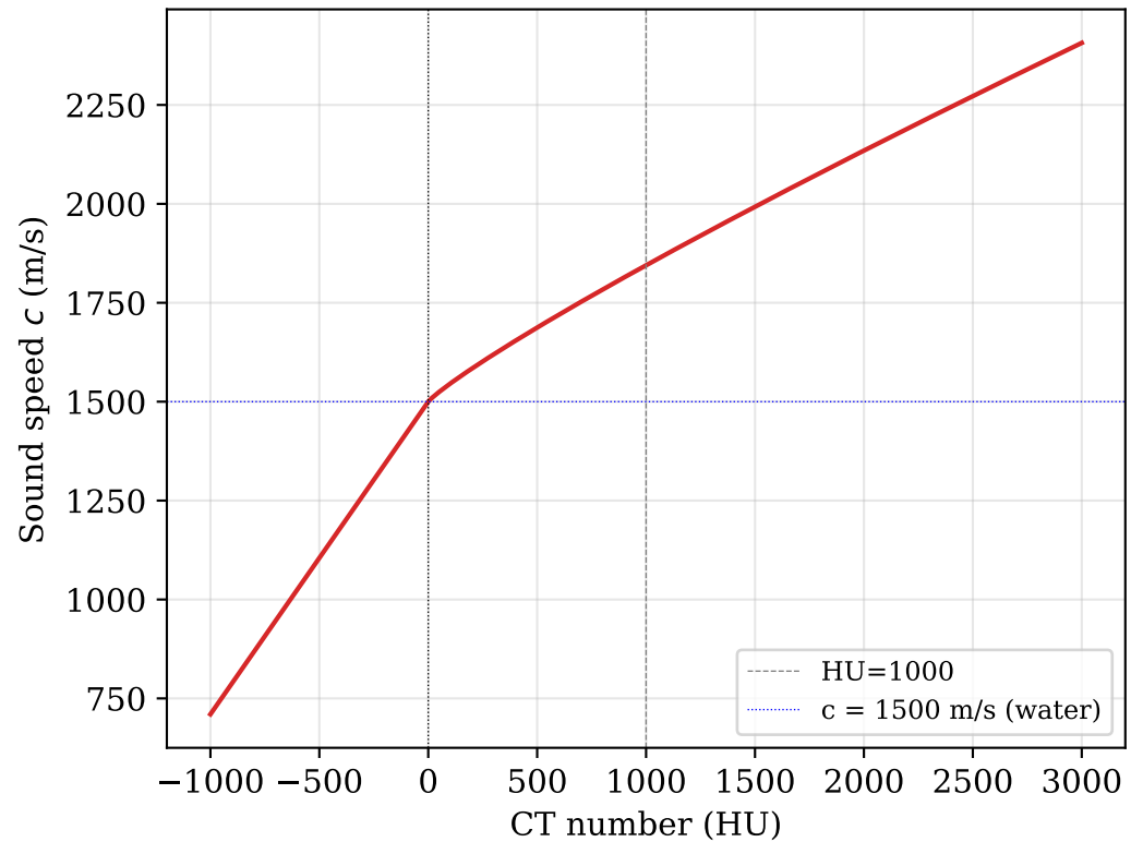
HU \rightarrow speed of sound (Schneider 1996)
