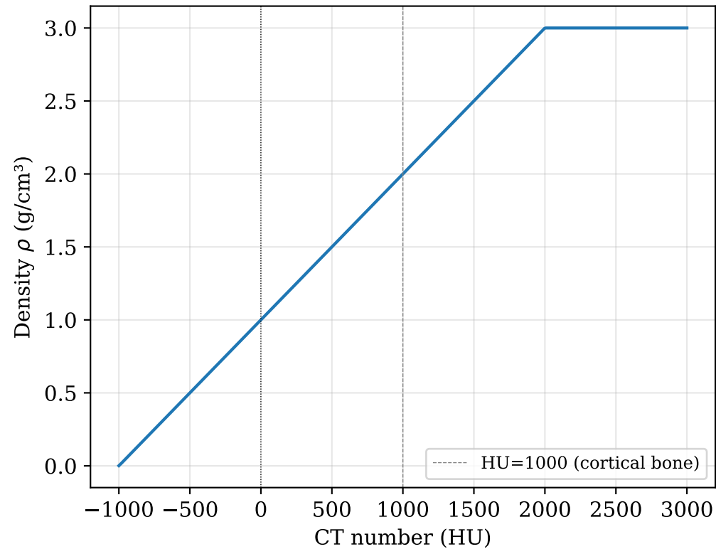
HU \rightarrow density
