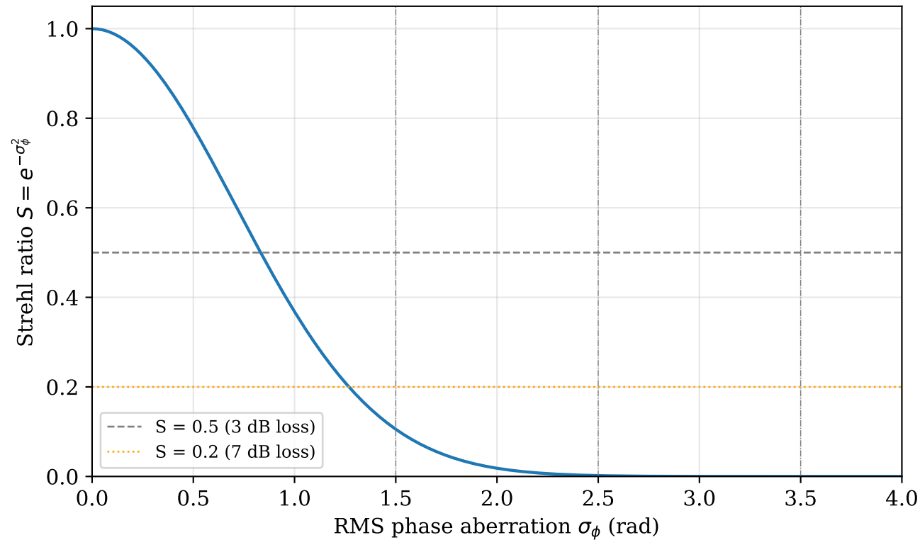
Transcranial focus degradation (Maréchal approximation)
