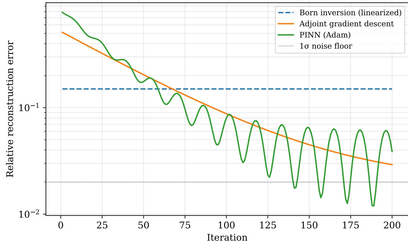
Convergence comparison: Born vs adjoint vs PINN
