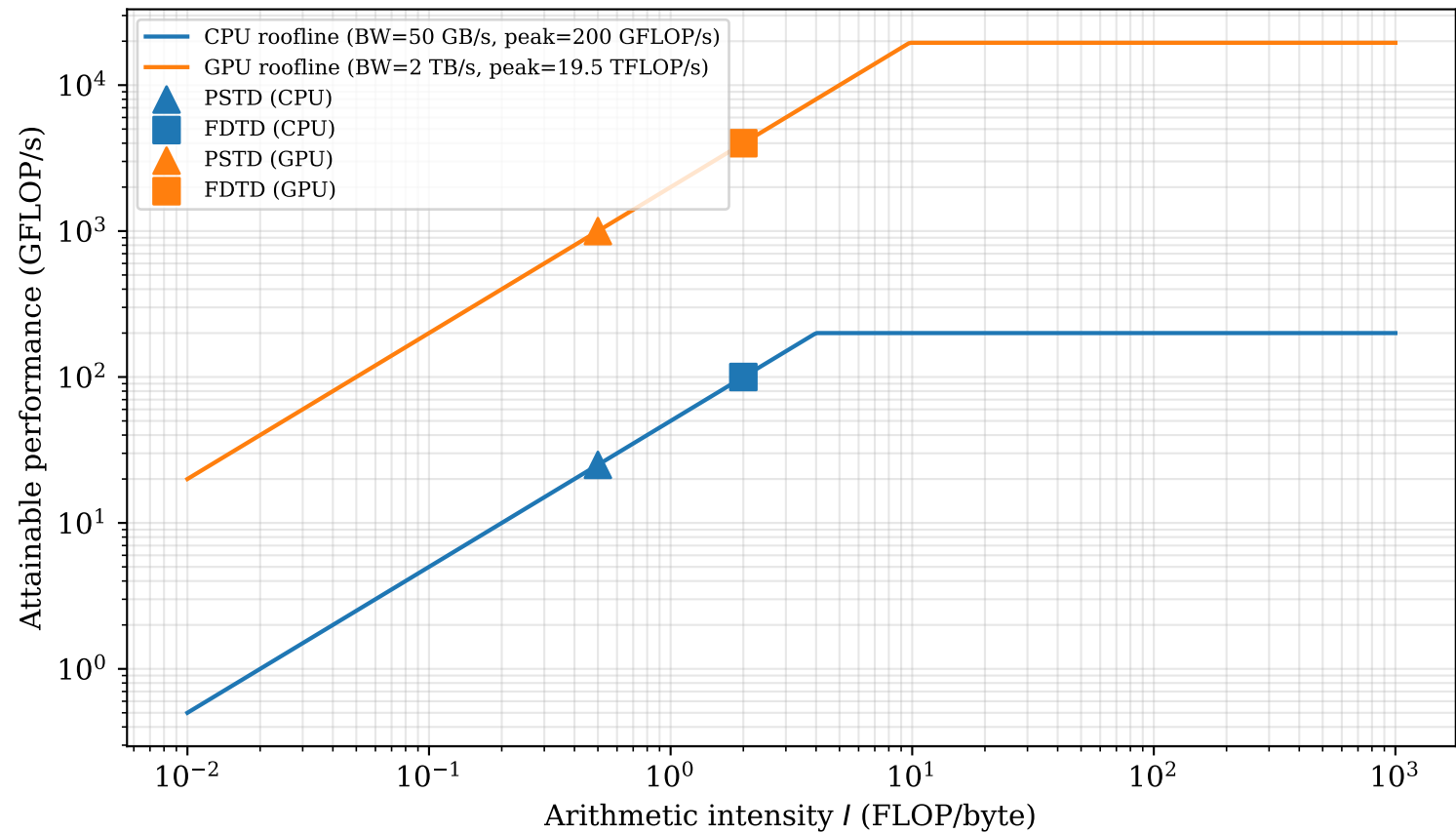
Roofline model for PSTD and FDTD
