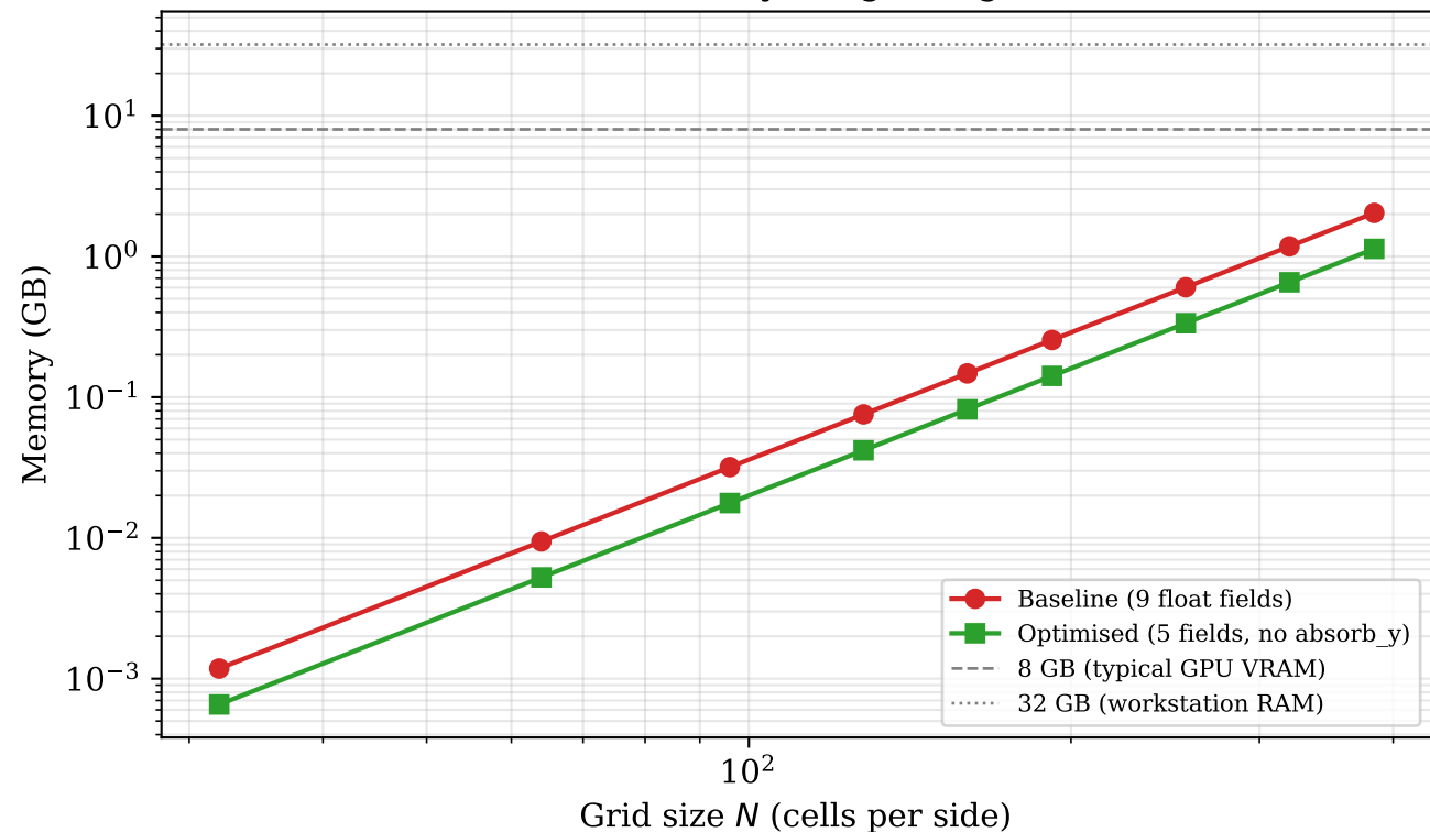
3D PSTD memory budget vs grid size
