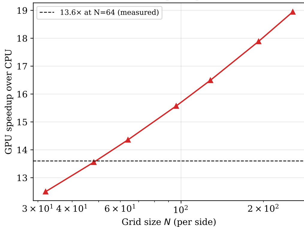
GPU/CPU speedup ratio
