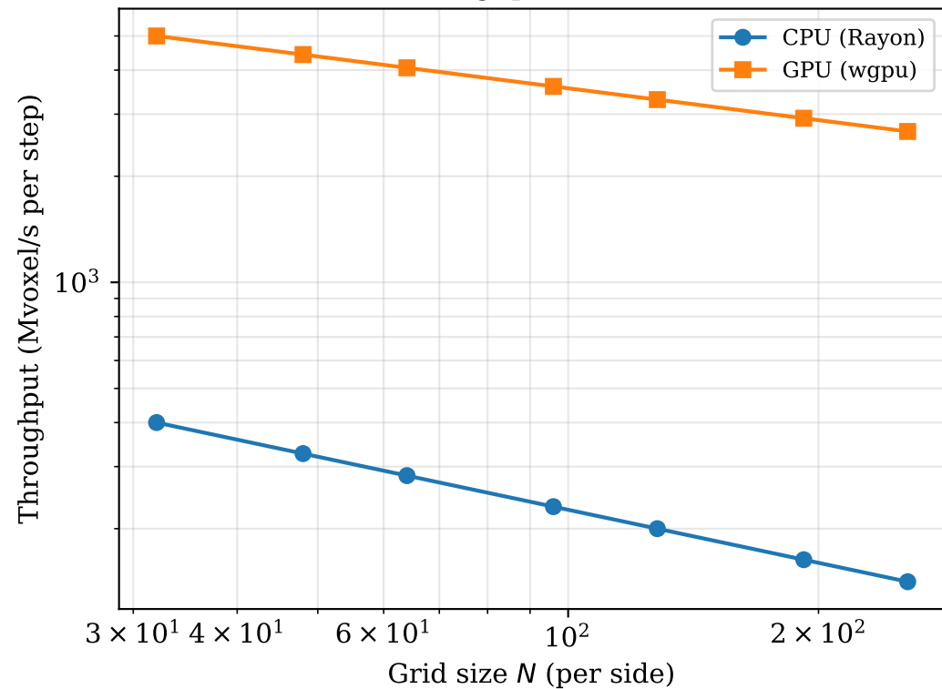
PSTD throughput: CPU vs GPU
