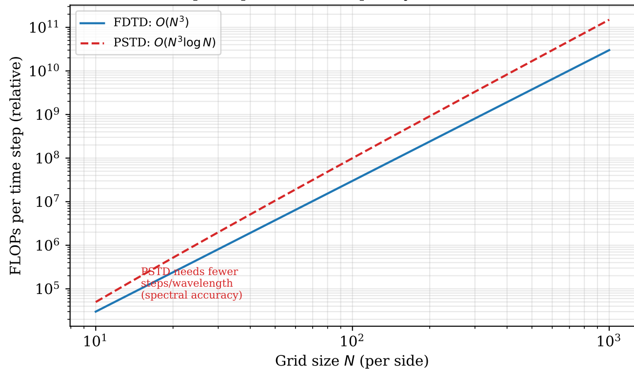
Per-step computational complexity: 3D FDTD vs PSTD
