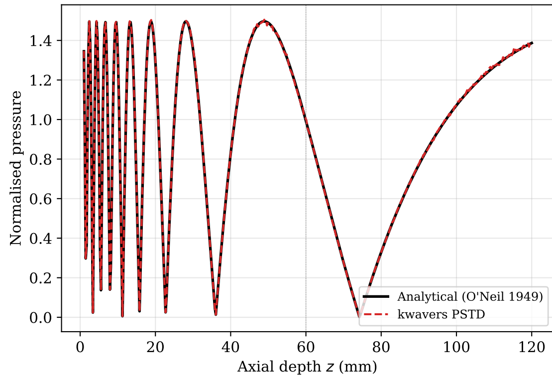
Focused bowl on-axis pressure r = 0.9999 , PSNR=49.6 dB
