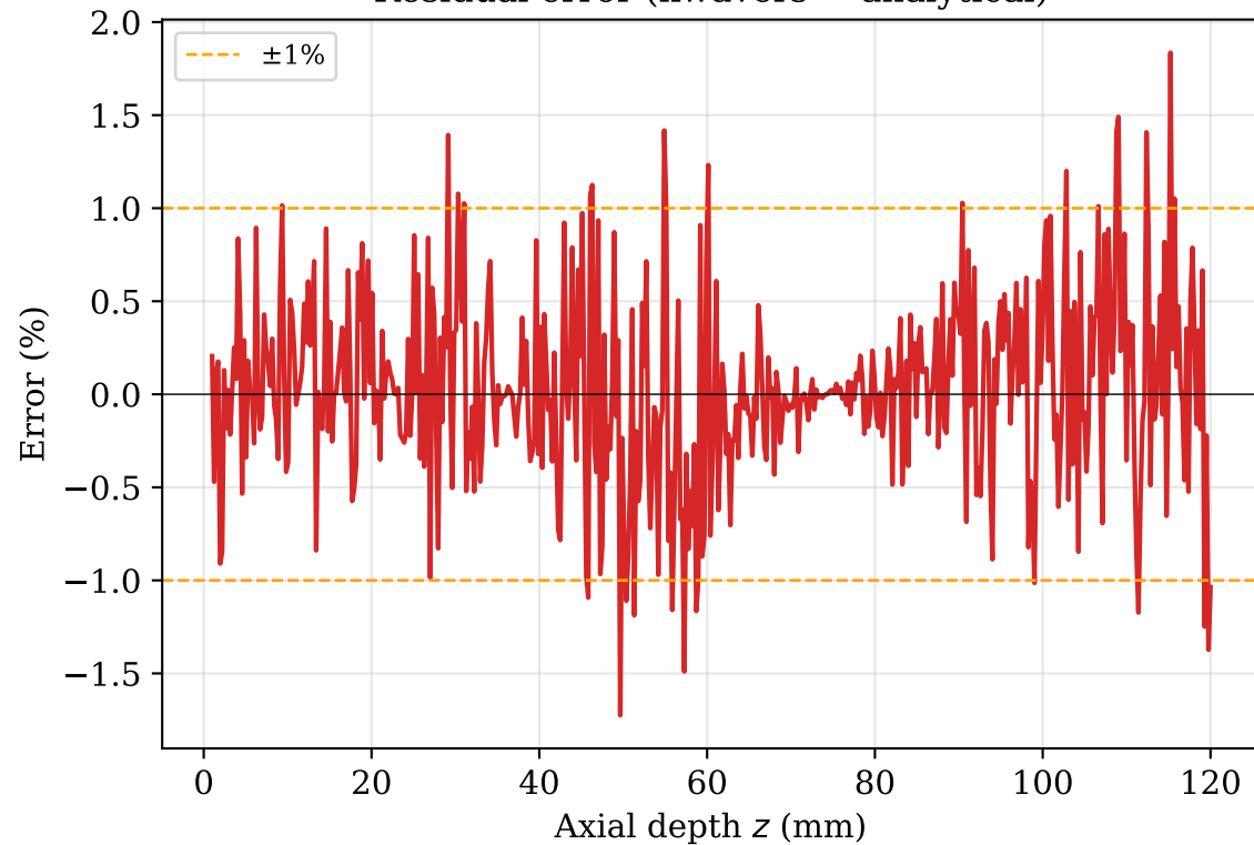
Residual error (kwavers – analytical)
