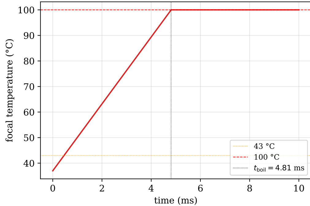
Millisecond, peak T = 100 °C
