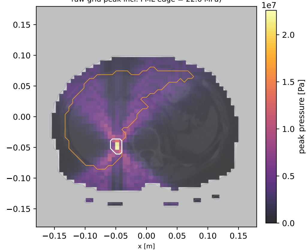
Focused-US in-body peak pressure = 22.6 MPa ( < 26 MPa intrinsic threshold — no cavitation isoline drawn; raw-grid peak incl. PML edge = 22.6 MPa)
