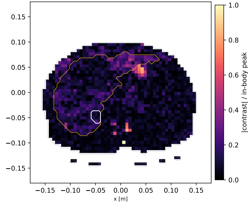
Reconstructed image (linearised Born, single-pass H^1 -Tikhonov) in-body peak = 0.195 (a.u.), multi-frequency imaging transmit, same aperture
