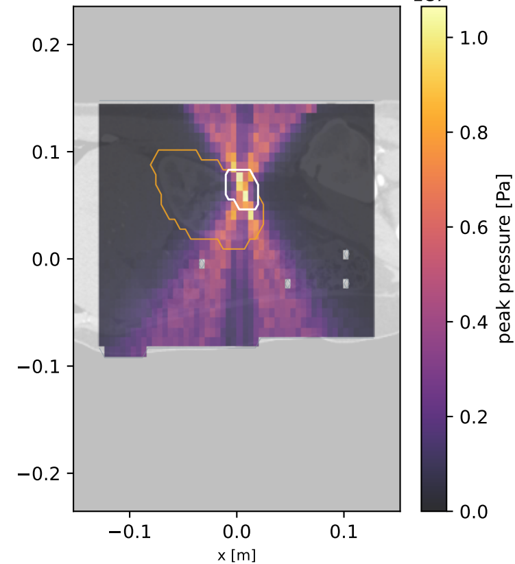
Focused-US in-body peak pressure = 10.7 MPa ( < 26 MPa intrinsic threshold — no cavitation isolate drawn; raw-grid peak incl. PML edge = 10.7 MPa) 1e7
