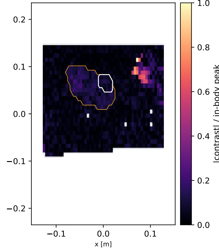
Reconstructed image (linearised Born, single-pass H^1 -Tikhonov) in-body peak = 0.304 (a.u.), multi-frequency imaging transmit, same aperture
