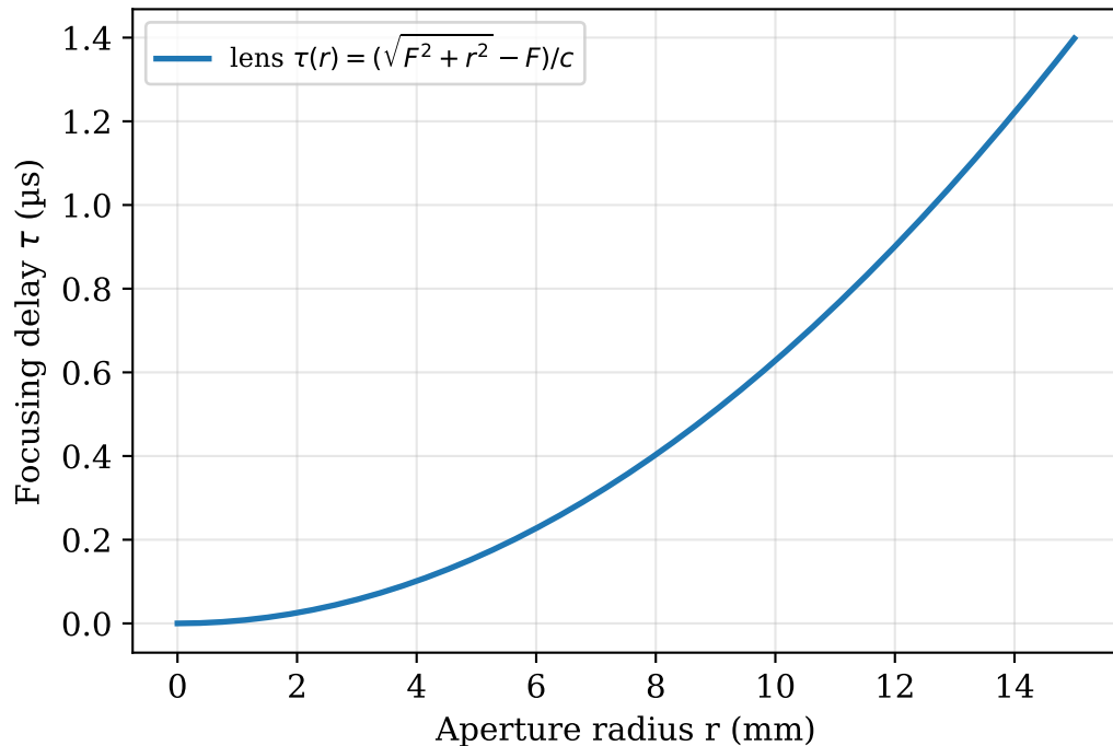
Static lens = passive delay law ( F = 50 mm)
