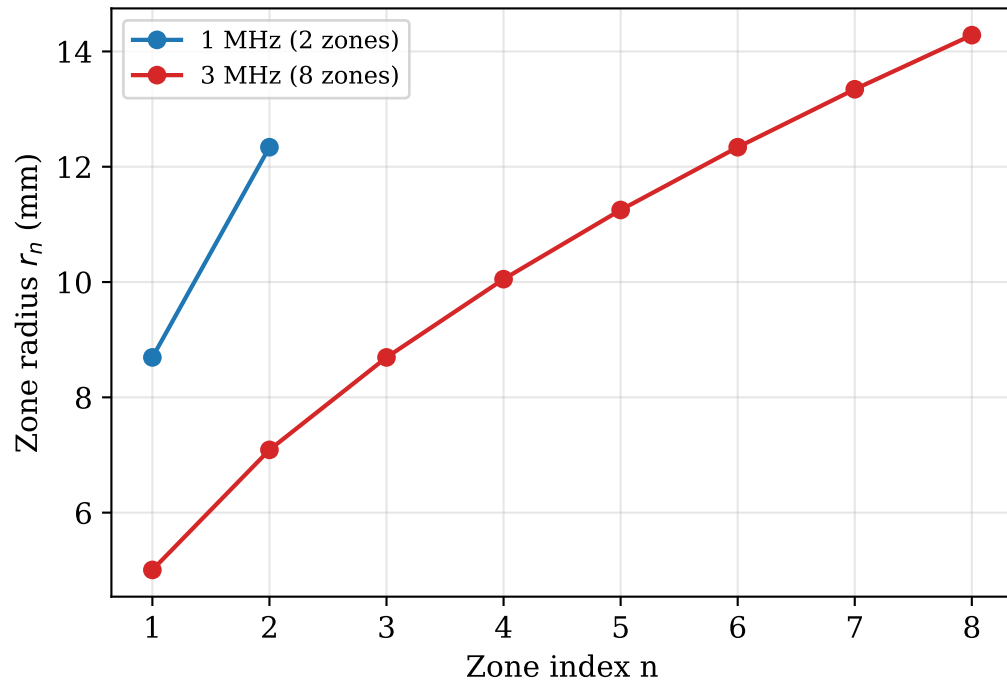
Fresnel zone plate: r_n = \sqrt{n\lambda F + (n\lambda/2)^2}
