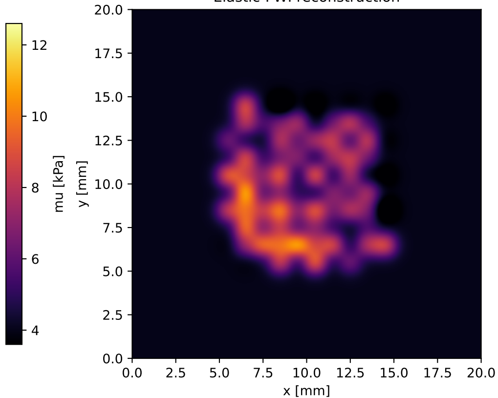
Elastic-FWI reconstruction
