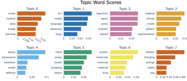
Fig. 6. Top c-TF-IDF keywords for representative discovered topics.
