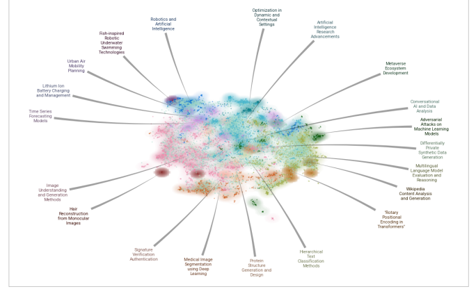
Fig. 4. Labeled topic landscape from 269,357 arXiv abstracts, visualized using stratified sampling (n=10,000) of UMAP reduced embeddings from BERTopic clustering.
