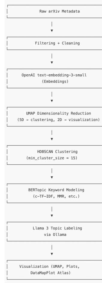
Fig. 1. Overall topic modeling pipeline from raw arXiv metadata to labeled topic visualizations.
