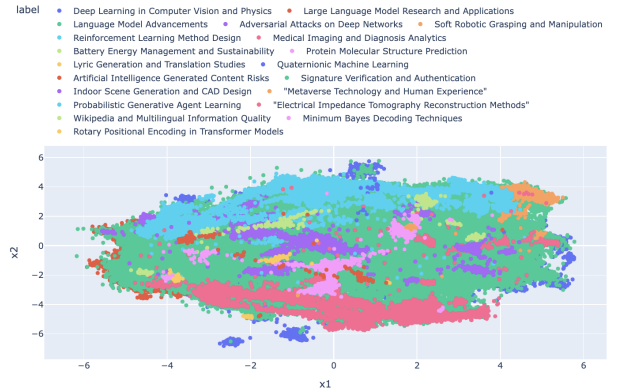
Fig. 5. UMAP scatter plot with topic assignments colored by LLM-generated labels.
