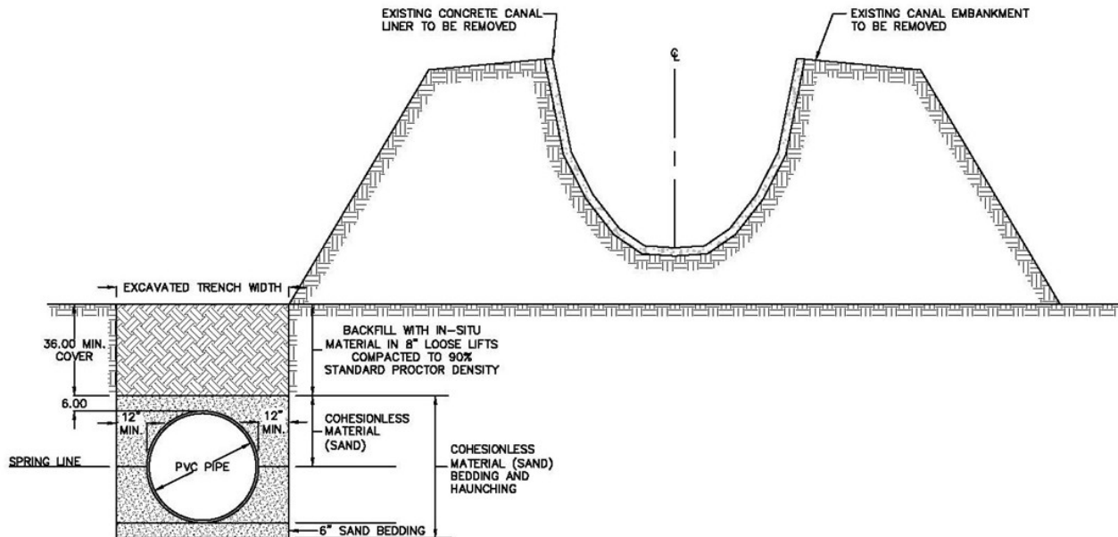
Pipeline Installation Typical Section.
