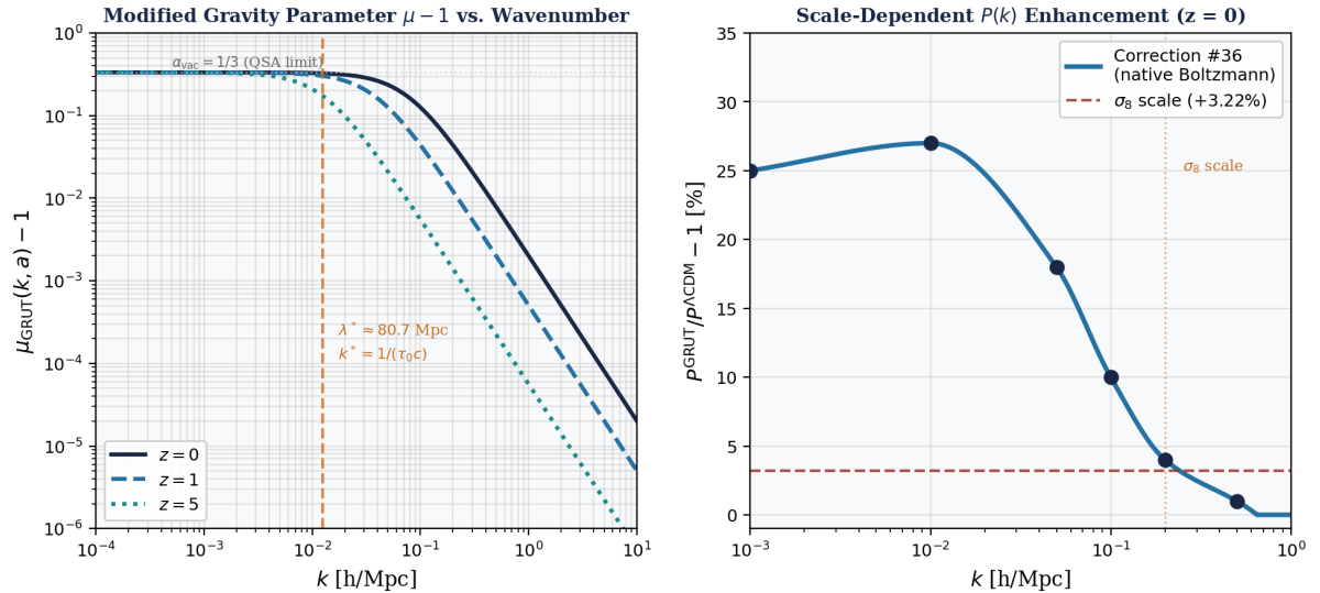
Figure 6. Kernel shape and scale-dependent growth response. Left: \mu_{\text{GRUT}}(k, a) - 1 as a function of wavenumber k at three redshifts ( z = 0, 1, 5 ). The Lorentzian profile peaks at super-horizon scales ( \mu - 1 \rightarrow 1/3 as k \rightarrow 0 ) and falls to sub-percent at the \sigma_8 scale ( k \sim 0.2\text{--}0.5 h/Mpc). Transition scale \lambda^* \approx 80.7 Mpc (marked). Note: the \mu \rightarrow 4/3 super-horizon limit is a formal limit of the QSA formula, not a derived relativistic asymptotic — see caveat above. Right: Scale-dependent P(k) enhancement at z = 0 from native Boltzmann injection (Correction #36). Enhancement ranges from +27% at k = 0.01 h/Mpc to +1% at k = 0.5 h/Mpc. The \sigma_8
