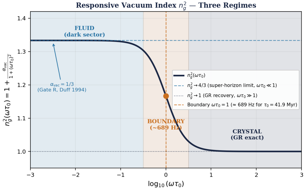
Figure 2. The three regimes of the CTP constitutive equation as a function of dimensionless frequency \omega\tau_0 . Left ( \omega\tau_0 \ll 1 ): fluid regime — n_g = \sqrt{4/3} , full dark-sector enhancement, galactic and cluster scales. Center ( \omega\tau_0 \approx 1 ): crystalline boundary — the decoherence plateau at \sim 689 Hz, primary falsifier. Right ( \omega\tau_0 \gg 1 ): crystal regime — n_g \rightarrow 1 , exact GR, GPS/LIGO/solar system. One curve, one medium, sixty orders of magnitude.
