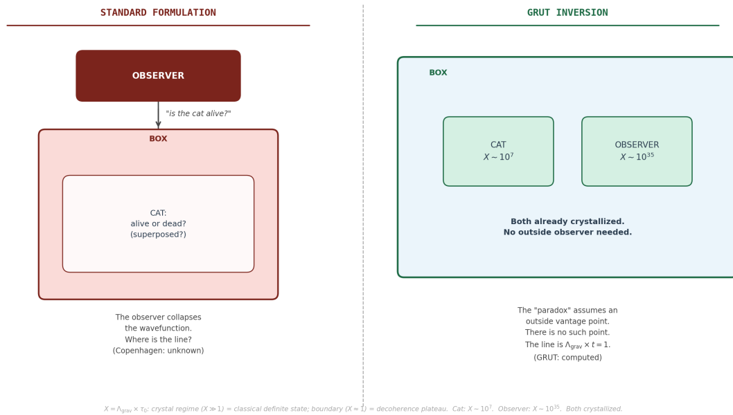
Figure 11. The GRUT inversion of Schrödinger's cat. Left (standard formulation): the observer stands outside the box and asks "is the cat alive?" — the wavefunction collapses on measurement, but Copenhagen cannot say where the observer–system line is. Right (GRUT
