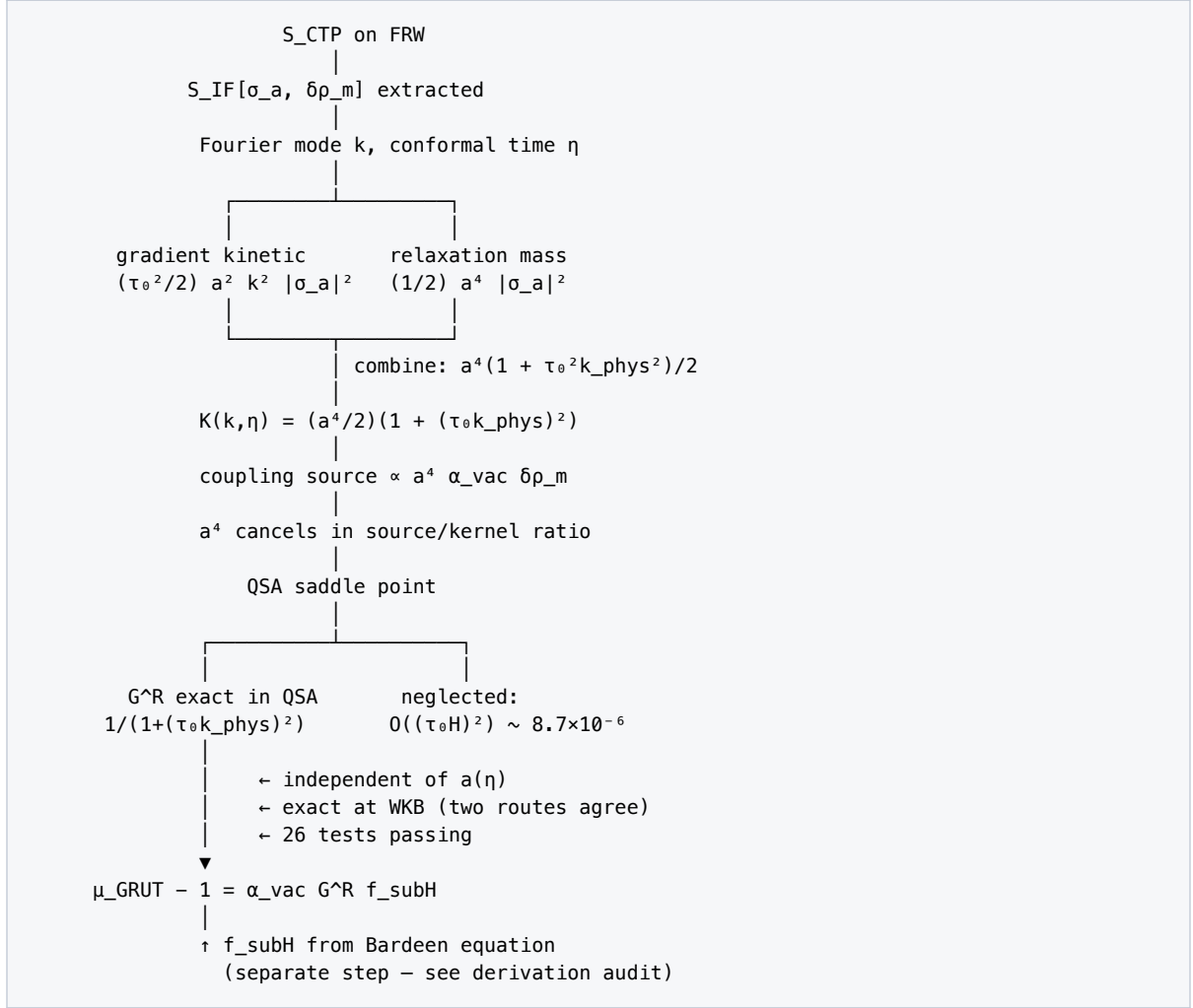
Figure 10. FRW Gaussian path integral derivation chain: S_{CTP} \rightarrow G^R(k_{phys}) . The influence functional S_{IF} on FRW (conformal time \eta , QSA) contains two quadratic terms in \sigma_a : gradient kinetic \propto a^2 k^2 and relaxation mass \propto a^4 . Combined kernel K = (a^4/2)(1 + (\tau_0 k_{phys})^2) . The coupling source \propto a^4 . In the Gaussian saddle-point ratio, a^4 cancels exactly — G^R acquires no a(\eta) dependence. The result G^R = 1/(1 + (\tau_0 k_{phys})^2) is exact in QSA (beyond-QSA corrections O((\tau_0 H)^2) \sim 8.7 \times 10^{-6} ). This figure documents Phase 2D (Correction #37, June 2026) — the derivation that promoted constitutive_growth_poisson_closure_gap from open to COMPUTED . The f_{subH} sub-Hubble filter enters from the Bardeen equation (logically distinct step; see Derivation Audit).
