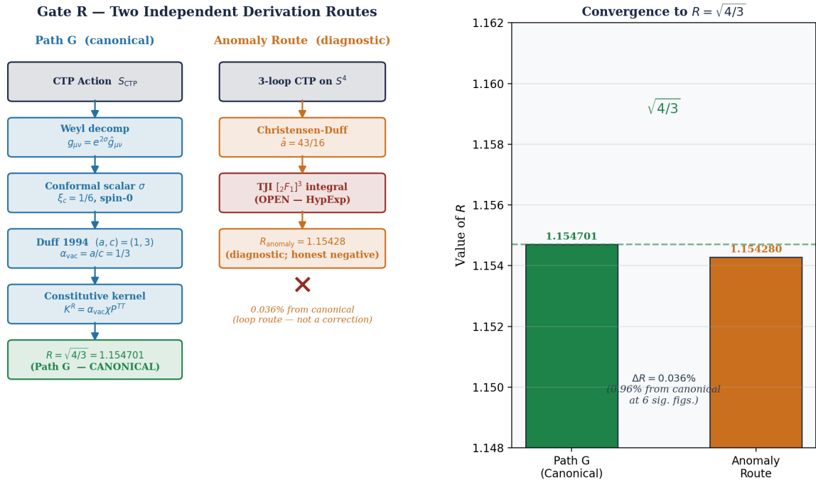
Figure 3. Two independent routes converging on R = \sqrt{4/3} \approx 1.15470 . Left (Path G, canonical): Weyl decomposition \rightarrow conformal scalar identification \rightarrow Duff 1994 a/c = 1/3 \rightarrow \alpha_{\text{vac}} = 1/3 \rightarrow n_g(o) = \sqrt{4/3} . Right (anomaly-quotient, diagnostic): 3-loop CTP on S^4 \rightarrow Christensen-Duff exact diagonal \hat{a} = 43/16 \rightarrow R_{\text{anomaly}} = 1.15428 (0.96% from canonical; honest negative). Osborn 2003 local-RG check gives \varepsilon = 1.15367 at M_Z , agreeing with canonical to 0.089% with no shared inputs.
