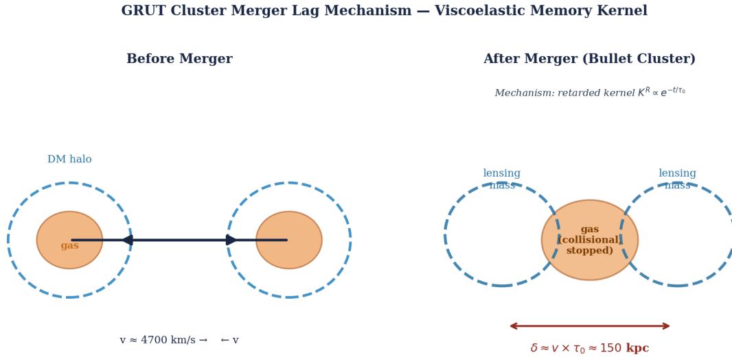
Figure 4. Schematic of the GRUT viscoelastic lag mechanism in a cluster merger. Left panel (pre-collision): two sub-clusters approaching with velocities v_1, v_2 ; gas (orange ellipses) and dark matter halo (blue shaded regions) are co-spatial. Right panel (post-collision): gas decelerates through ram-pressure interaction while lensing mass (tracking the memory-kernel-lagged response) continues forward; offset \delta \approx v_{\text{post}} \times \tau_0 \times \text{dec\_ratio} opens between gas centroid and lensing peak. The 41.9 Myr retarded kernel is the sole new physics — no additional fields or fitted parameters.
