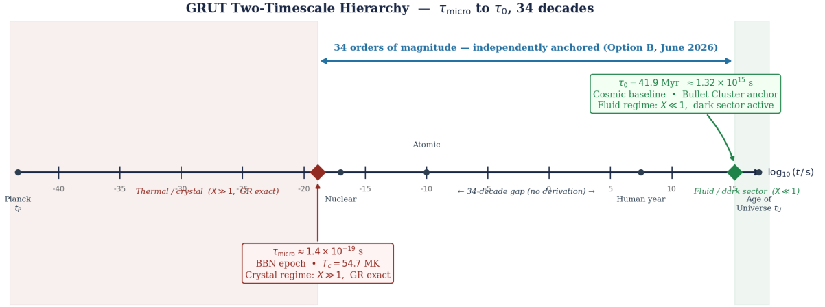
Figure 1. Logarithmic timescale map spanning 34 orders of magnitude. The microscopic thermal scale \tau_{\text{micro}} \approx 1.4 \times 10^{-19} \text{ s} (anchored by T_c = 54.7 \text{ MK} via \hbar/k_B T_c ) governs the vacuum's phase transition. The macroscopic gravitational scale \tau_0 = 41.9 \text{ Myr} (anchored by the cosmic baseline and Bullet Cluster offset) governs every cosmological prediction. Both are independently anchored; no derivation between them exists in the current framework (Option B, June 2026).
