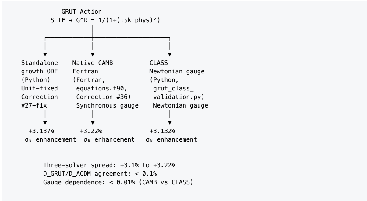
Figure 11. Triple-convergence validation of the GRUT \sigma_8 growth response. Three independent implementations — a Python standalone growth ODE (Correction #27 + unit fix), native CAMB 1.5.8 Fortran (Correction #36), and a Python CLASS+ODE in Newtonian gauge — produce the same \sigma_8 enhancement to within 0.1%. The three implementations share no code, use different gauge choices (synchronous vs. Newtonian), and run on different \Lambda CDM backgrounds (CAMB vs. CLASS). The growth-factor ratio D_{\text{GRUT}}/D_{\Lambda\text{CDM}} is gauge-background-independent to < 0.01\% . The 0.09% spread (3.137% vs 3.22%) reflects the difference between quasi-static-approximation ODE and full self-consistent Boltzmann integration; both are correct in their respective regimes. Independent solver, independent gauge, independent codebase — one answer.
