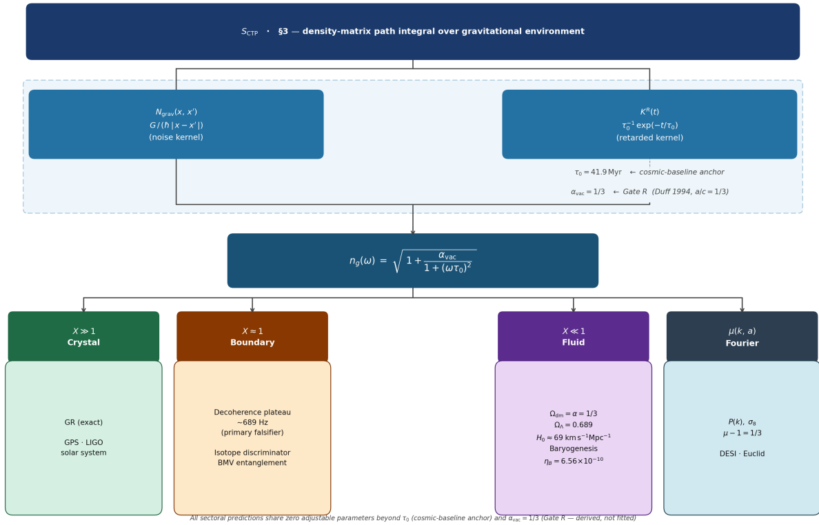
Figure 10. The complete GRUT derivation chain. S_{CTP} (§3) produces two kernels — N_{grav}(x, x') = G/(\hbar|x-x'|) (noise kernel) and K^R(t) = \tau_0^{-1} \exp(-t/\tau_0) (retarded kernel) — which together determine \tau_0 = 41.9 \text{ Myr} (cosmic-baseline anchor) and \alpha_{vac} = 1/3 (Gate R, Duff 1994 a/c = 1/3 ). These produce the refractive index n_g(\omega) from which four regime branches descend: Crystal ( X \gg 1 ): GR exact, GPS, LIGO. Boundary ( X \approx 1 ): decoherence plateau ~689 Hz (primary falsifier), isotope discriminator, BMV entanglement. Fluid ( X \ll 1 ): \Omega_{dm} = \alpha = 1/3 , \Omega_\Lambda = 0.689 , H_0 \approx 69 \text{ km/s/Mpc} , \eta_B = 6.56 \times 10^{-10} . Fourier \mu(k, a) : P(k) , \sigma_8 , \mu - 1 = 1/3 (DESI/Euclid). Zero free parameters beyond \tau_0 and \alpha_{vac} .
