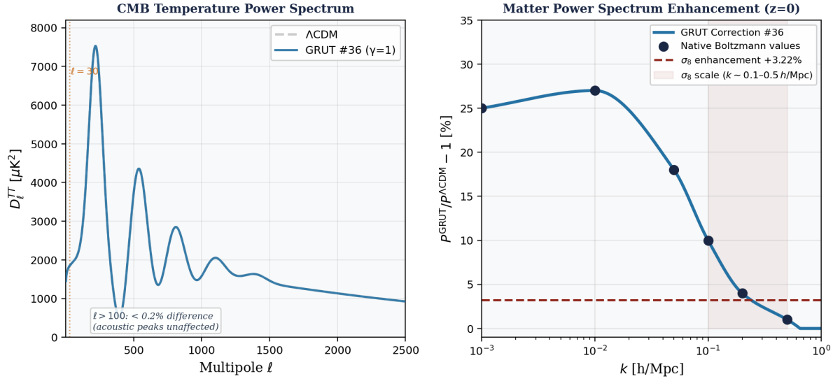
Figure 7. CMB spectrum and matter power spectrum from native Boltzmann injection (Correction #36). Left: Schematic CMB temperature power spectrum D_l^{TT} — GRUT (blue) vs. \Lambda CDM (dashed black). The Correction #36 native Fortran implementation leaves metric evolution unmodified ( \gamma = 1 ); low- l behavior is schematic — for the diagnosed prototype excess see Figure 8. Acoustic peaks ( l \geq 100 ) unaffected at < 0.2\% . Right: P(k) ratio P^{GRUT}/P^{\Lambda CDM} at z = 0 from native Boltzmann injection (Correction #36). Enhancement ranges from +27% at k = 0.01 h/Mpc to +1% at k = 0.5 h/Mpc ; \sigma_8 enhancement +3.22% (Correction #36 native Fortran). For comparison, the prototype Poisson-constraint run (Figure 8) shows +48% at k = 0.003 h/Mpc — a diagnosed etak/z mismatch artifact. Three-solver consensus \sigma_8 enhancement: +3.1% (see Figure 11 for triple-convergence validation). Both panels use Planck 2018 parameters.
