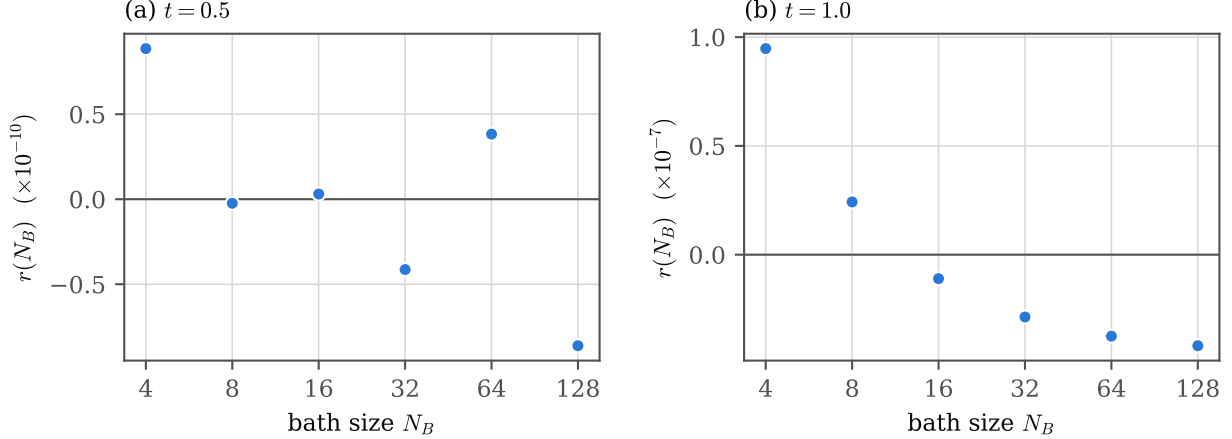
Figure 3: Normalised residual r(N_B) = N_B \gamma_1(N_B) / \langle N_B \gamma_1 \rangle - 1 , with \langle \cdot \rangle the mean over the bath-size grid, of the ramp-protocol force at (a) t_\star = 0.5 and (b) t = 1.0 . Authoritative numerical output. The panels have independent vertical scales. At t_\star the residuals scatter at the level of the computation’s numerical precision, so no finite- N_B correction is resolved; at t = 1.0 a monotone correction is resolved.
