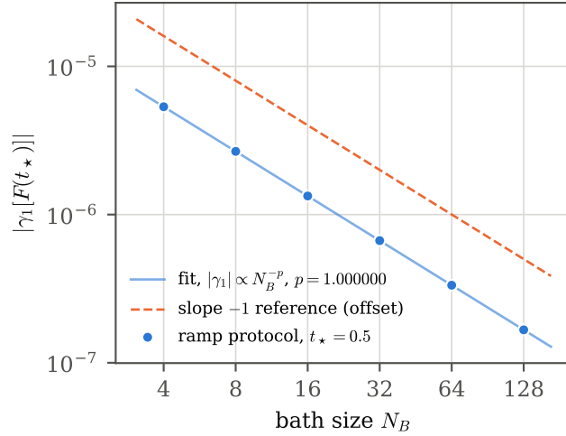
Figure 2: Standardised skewness of the ramp-protocol force at t_* = 0.5 against bath size, on logarithmic axes. Points: authoritative numerical output. Solid line: least-squares power law, p = 1.000000 . Dashed line: slope -1 , offset vertically for visibility. The time t_* is not claimed to lie inside the theorem's window.
