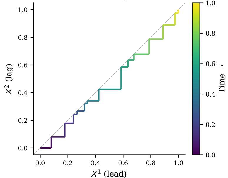
(c) Phase space
