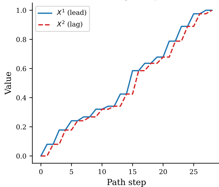
(b) Lead / Lag components
