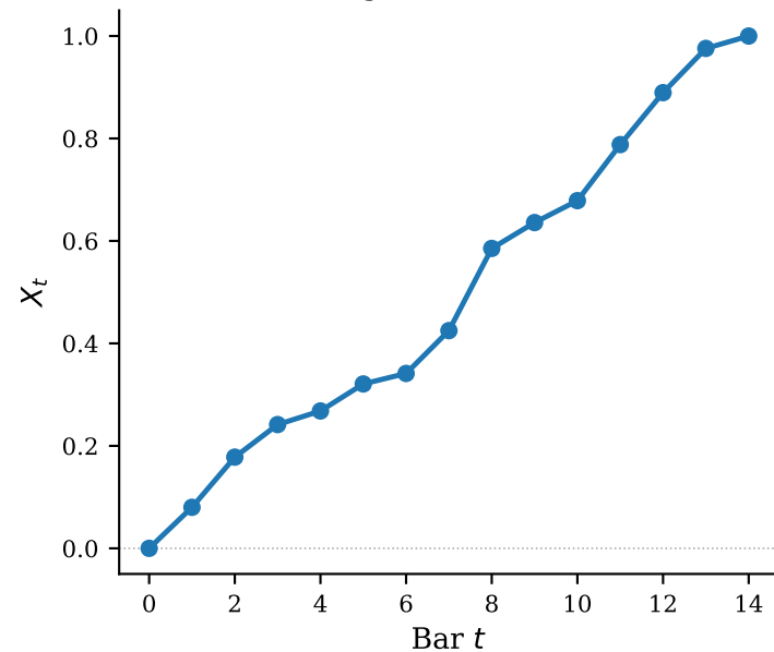
(a) Original time series
