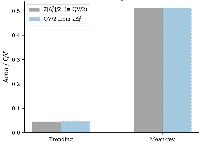
(b) Total triangle area = \frac{1}{2} QV (identity check)
