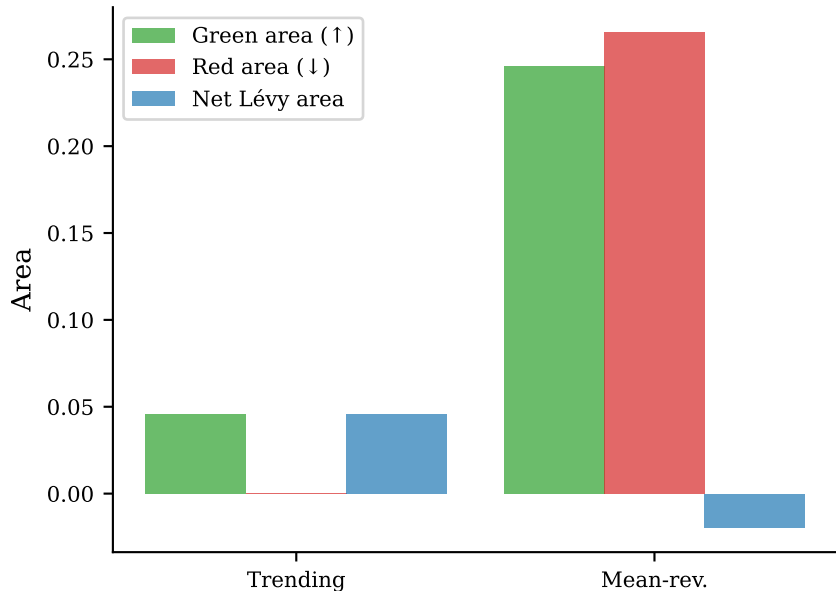
(a) Signed-area decomposition
