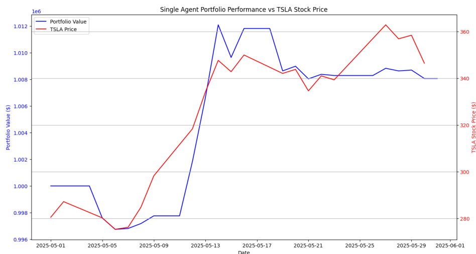
Figure: Single Agent Implementation Experiment on TSLA for May 2025
