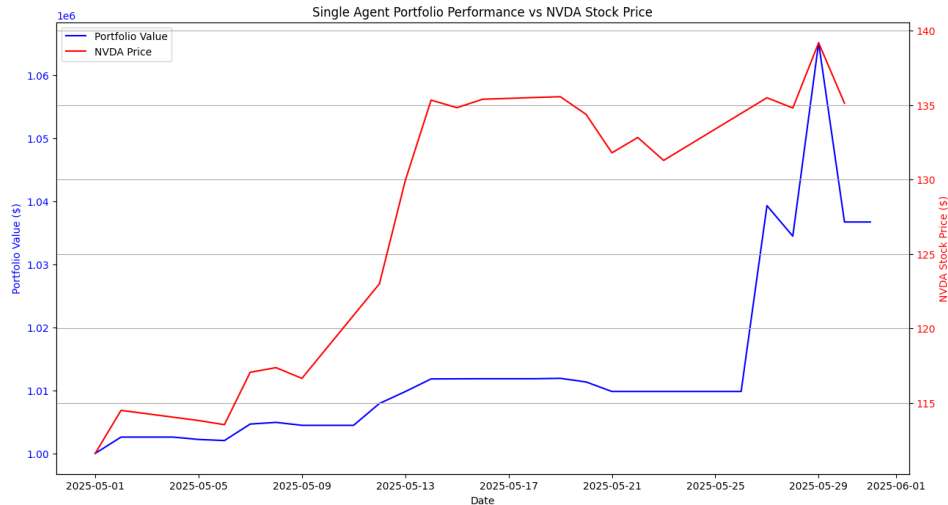
Figure: Single Agent Implementation Experiment on NVDA for May 2025
