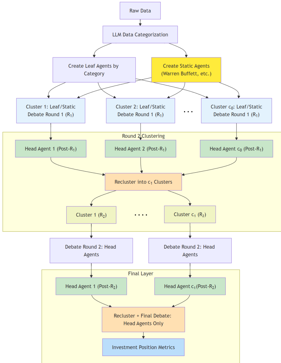
Figure: Example Flowchart of Agent Orchestration.
