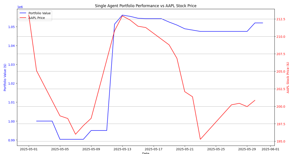
Figure: Single Agent Implementation Experiment on AAPL for May 2025
