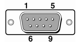
RS232 DB9 Male Projector
