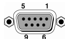
RS232 DB9, Female
