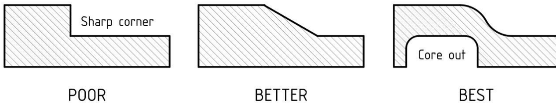
Figure 2.4: Thickness transition guide. Inspired by DuPont Engineering Polymers (2000).
