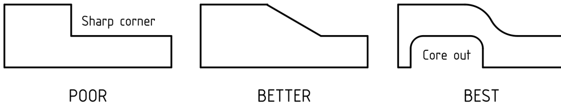
Figure 2.4: Thickness transition guide
