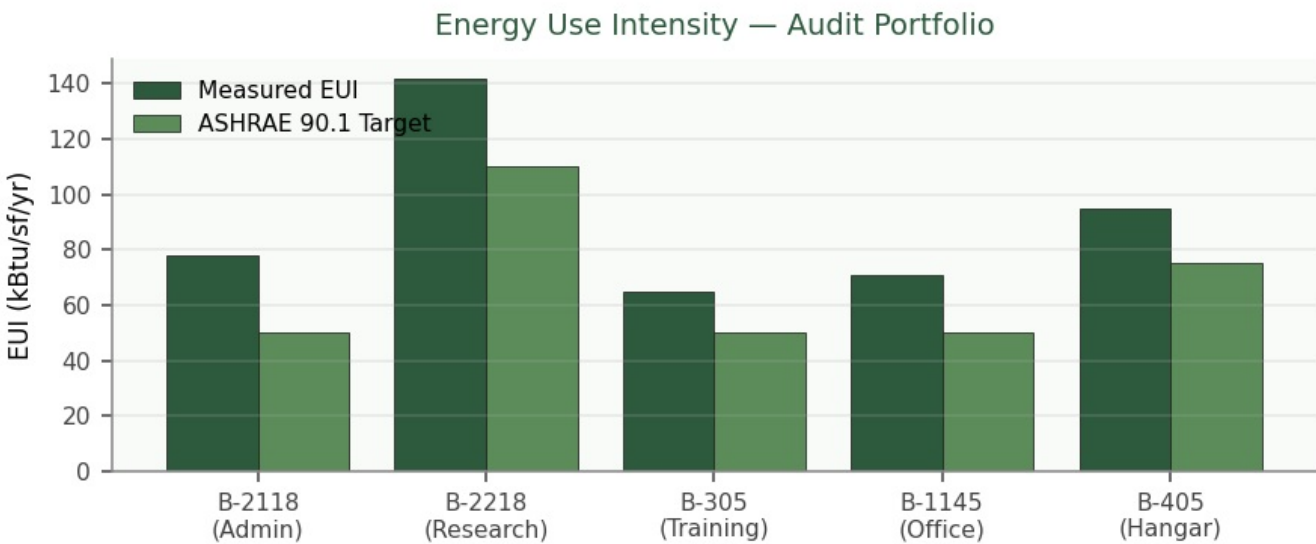
Figure 1. Energy Use Intensity — Audit Portfolio Buildings
