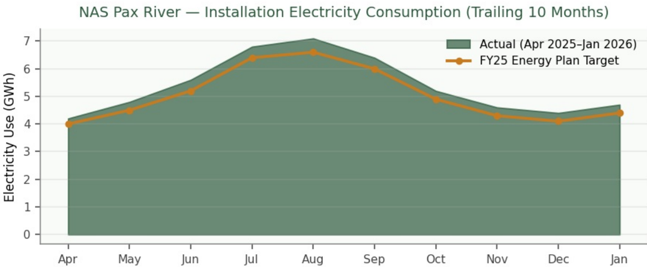
Figure 1. Installation Electricity Consumption — Trailing 10 Months
