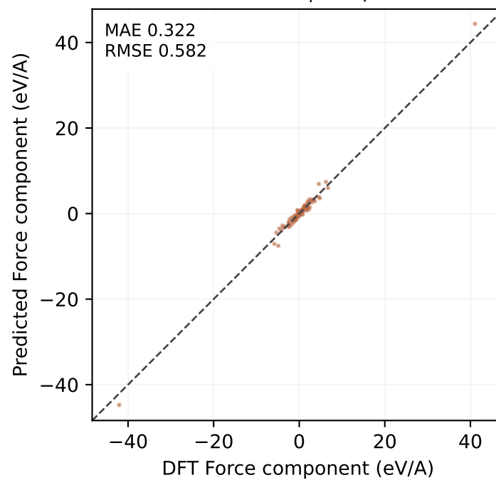
MP-ALOE test | 180 points
