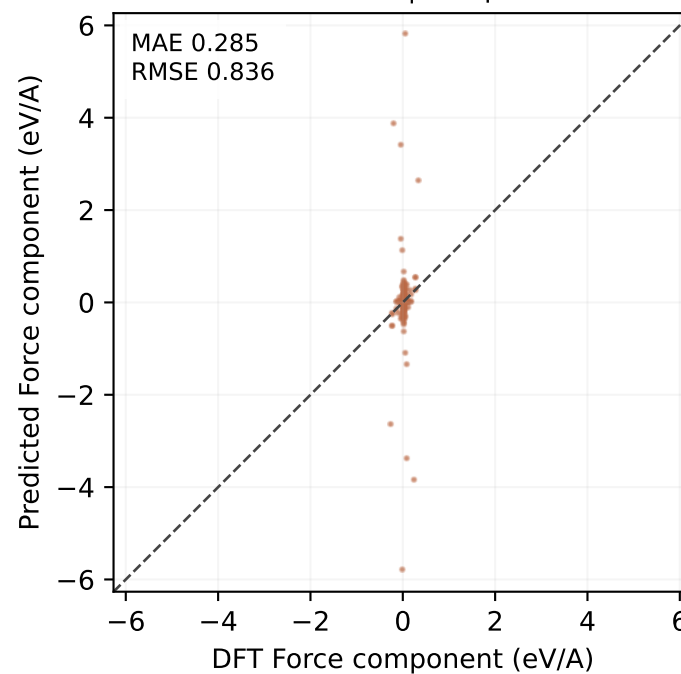
MP-ALOE test | 180 points
