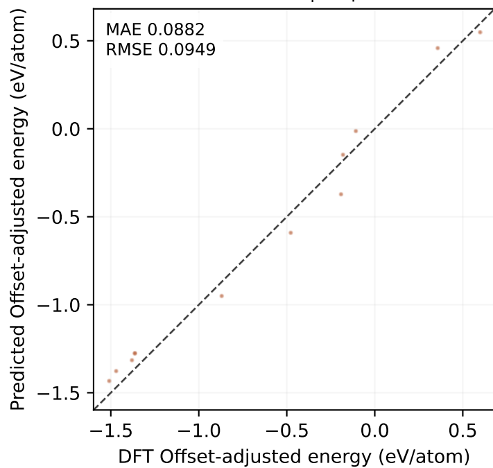
MP-ALOE test | 12 points
