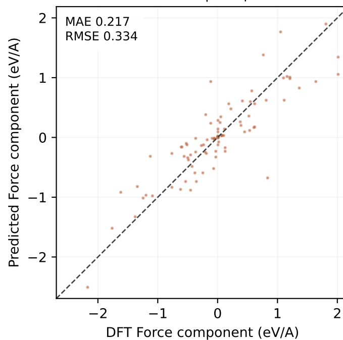
MP-ALOE test | 693 points
