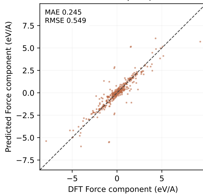
MP-ALOE test | 693 points
