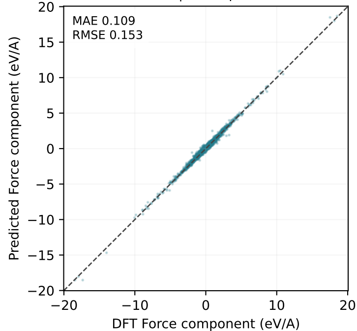
MatPES test | 114 points
