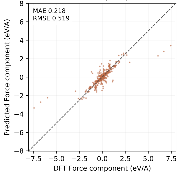
MP-ALOE test | 540 points
