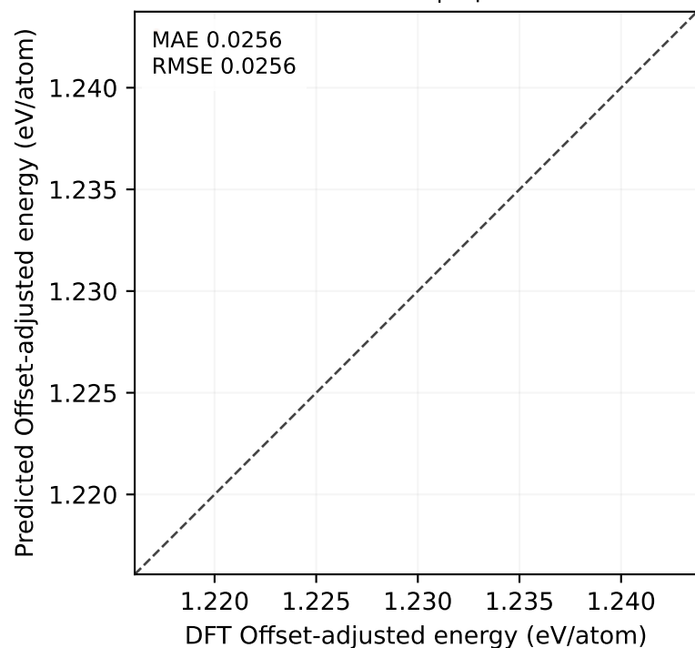
MatPES test | 1 points
