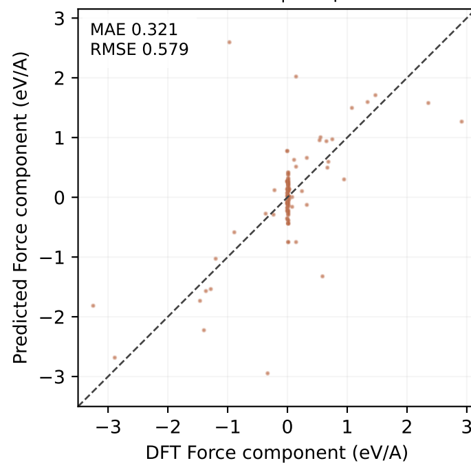
MP-ALOE test | 648 points
