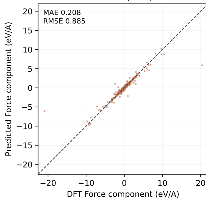
MP-ALOE test | 648 points
