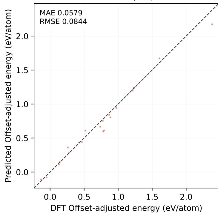
MP-ALOE test | 21 points
