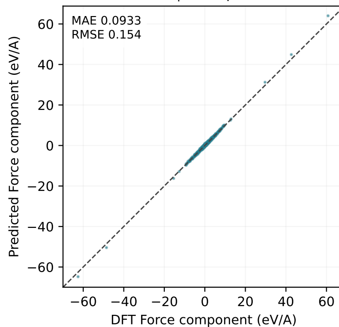
MatPES test | 1,152 points
