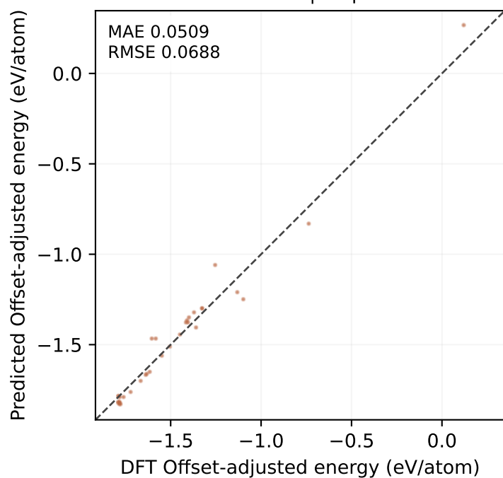
MP-ALOE test | 24 points
