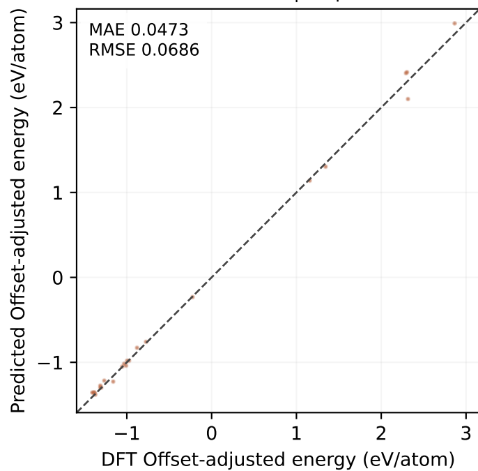
MP-ALOE test | 24 points
