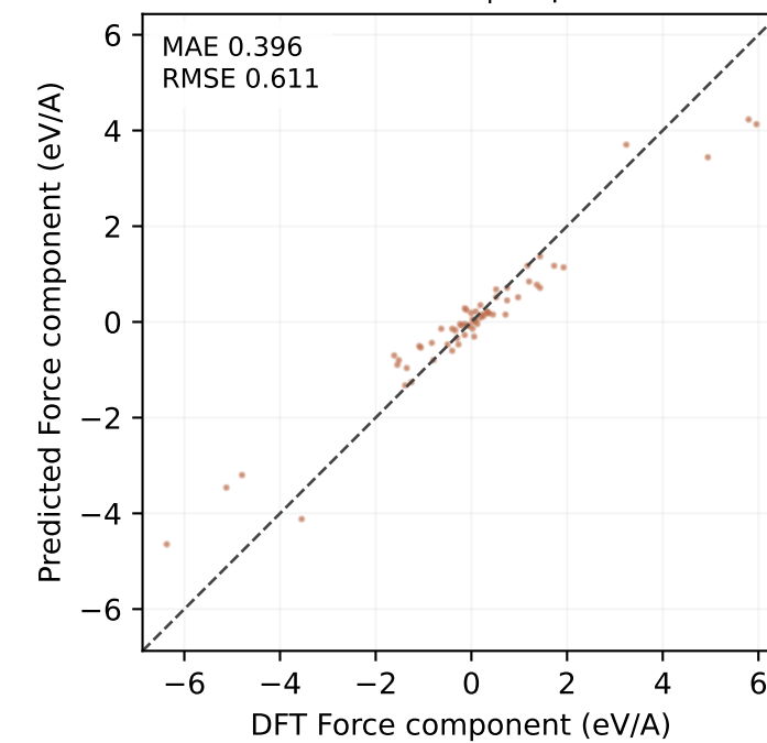
MP-ALOE test | 63 points
