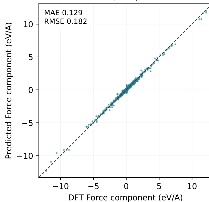
MatPES test | 378 points
