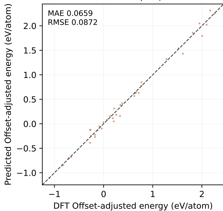
MP-ALOE test | 39 points
