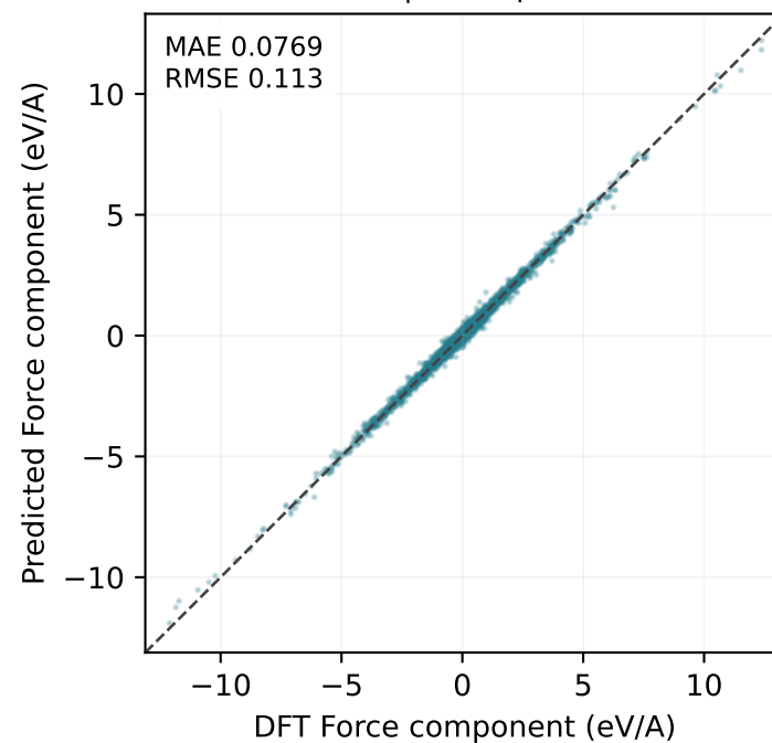
MatPES test | 360 points
