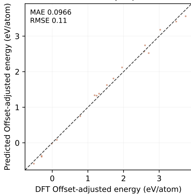
MP-ALOE test | 18 points
