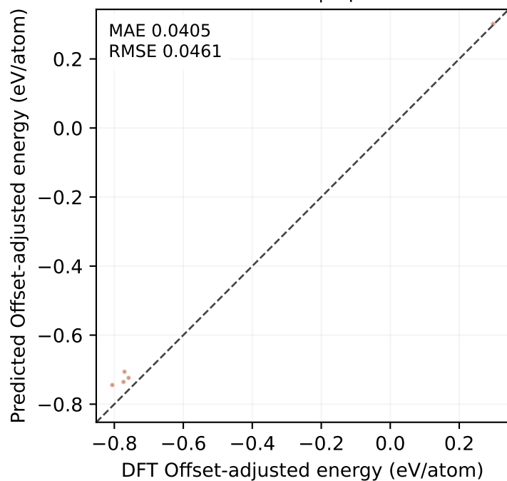
MP-ALOE test | 18 points
