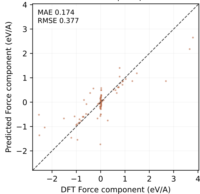
MP-ALOE test | 288 points
