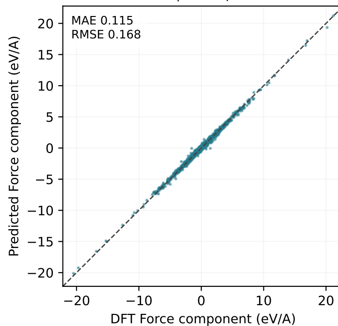
MatPES test | 180 points
