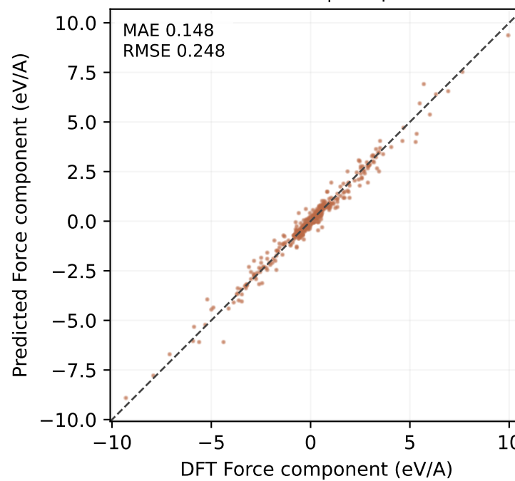
MP-ALOE test | 675 points
