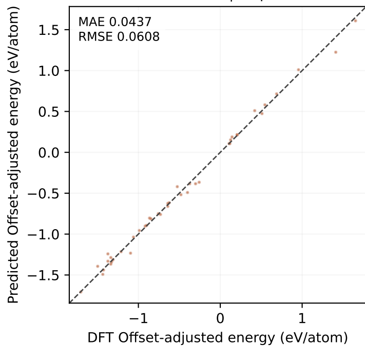
MP-ALOE test | 42 points
