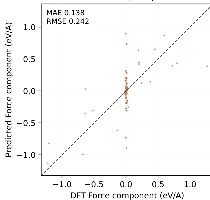
MP-ALOE test | 675 points
