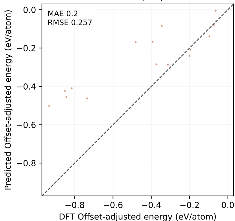
MatPES test | 15 points
