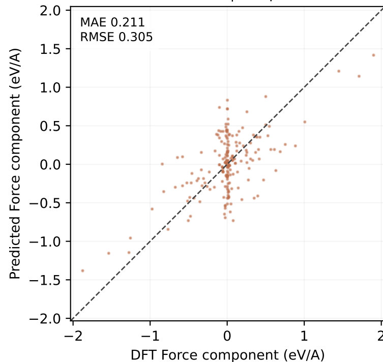
MatPES test | 252 points
