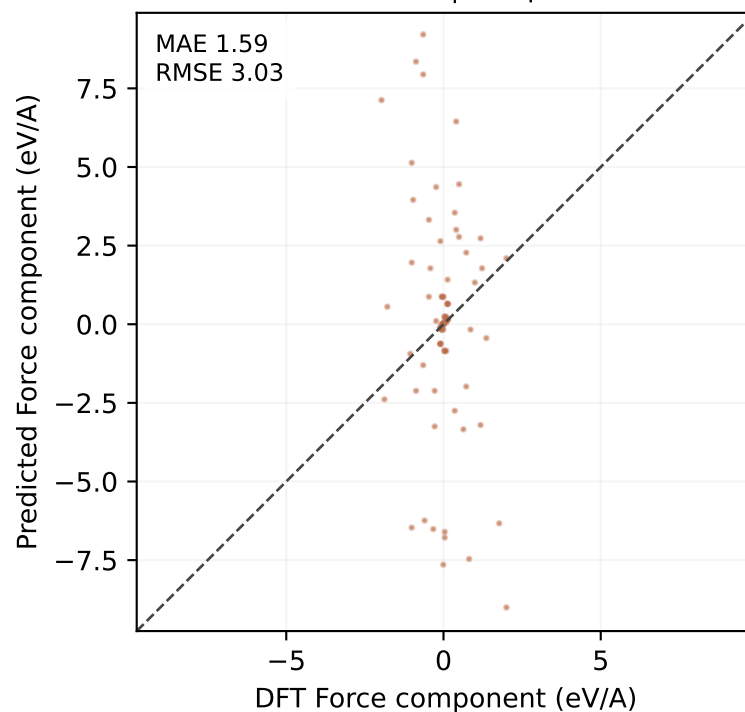
MatPES test | 123 points
